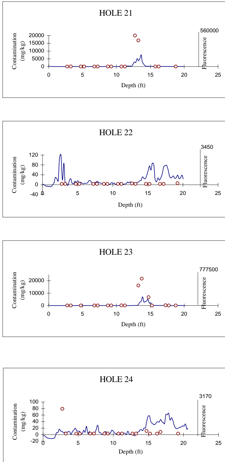
Figure 6-4. Adjusted downhole results for Port Hueneme. This figure provides a summary of all downhole results after adjustment for depth measurement inaccuracies due to sloughing that appears to have affected the measurements in the saturated zone at boring locations 23 and 28. Note that the vertical axes for the holes beyond the plume boundary, holes 22, 24, and 27, have a smaller scale than holes 21, 23, 25, 26, and 28, where contamination was detected.
