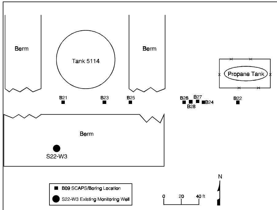
Figure 5-2. Demonstration site and sampling locations, Port Hueneme. B21-B28 are the locations of the HSA borings associated with the CPT pushes. For example, B21 is the boring associated with PHDP21, the initial SCAPS push.
