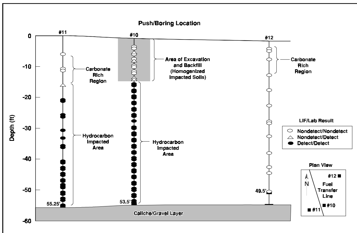
Figure 6-9. Subsurface contaminant map for SNL Tank Farm. Cross-section view of the results shown in Table 6-3, comparing the ATI results to those of the SCAPS LIF. The results are based on the adjusted downhole data shown in Figure 6-8.
