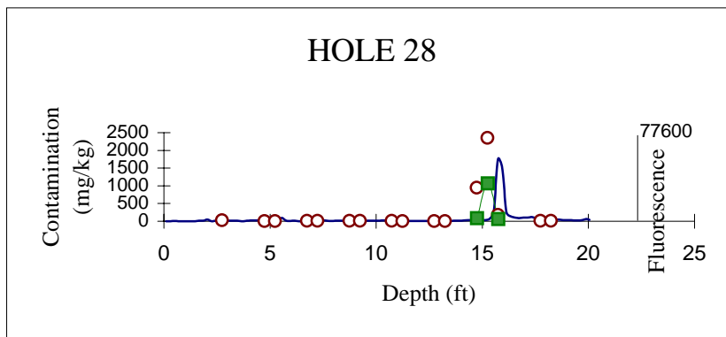
Figure 6-3. Downhole results for Port Hueneme. (Continued)
