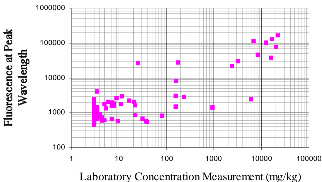
Figure 6-2. Plot of results of comparison of Port Hueneme LIF data with laboratory data.
