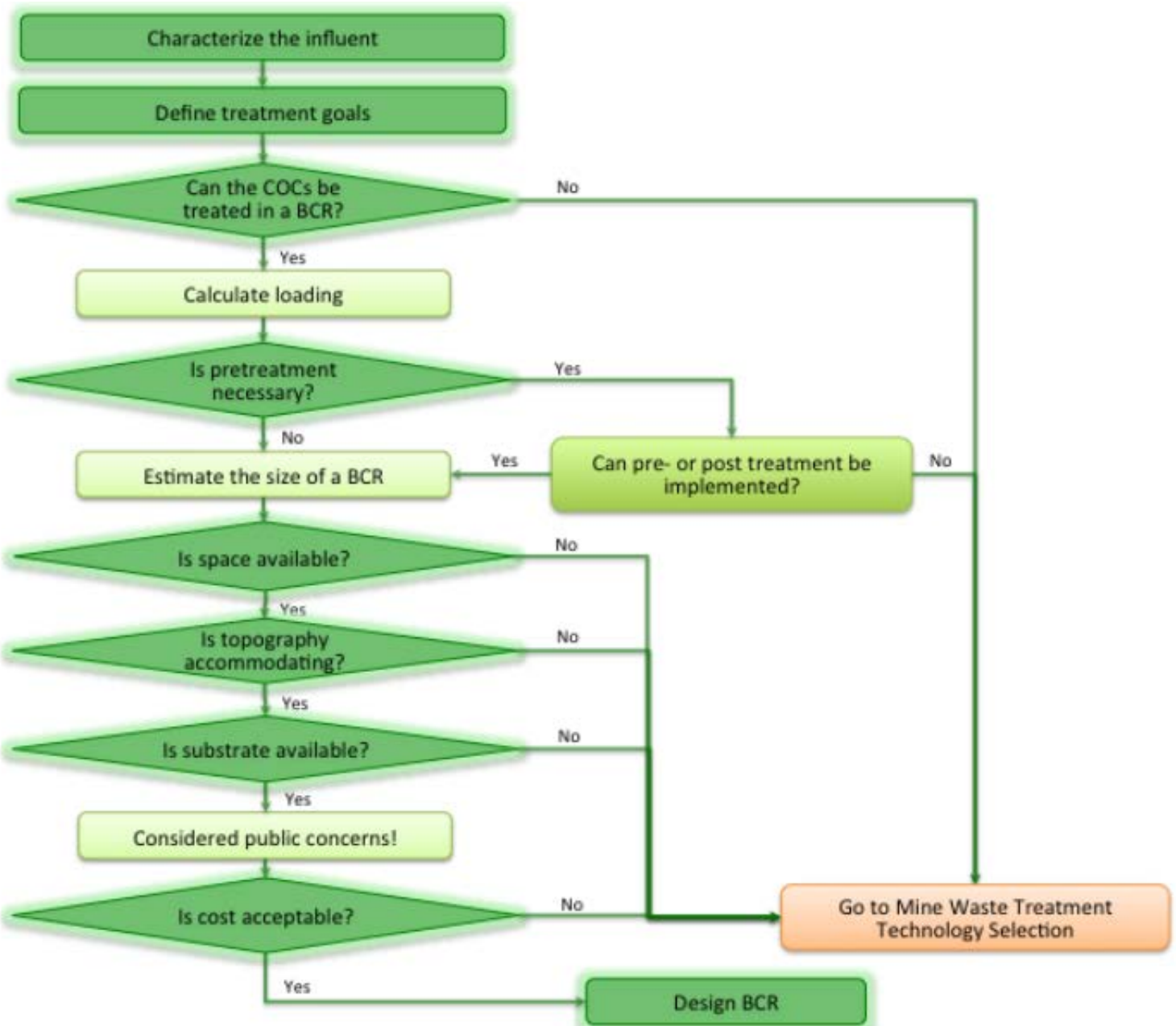
Figure 2-1. Decision flow process for determining the applicability of a biochemical reactor.
