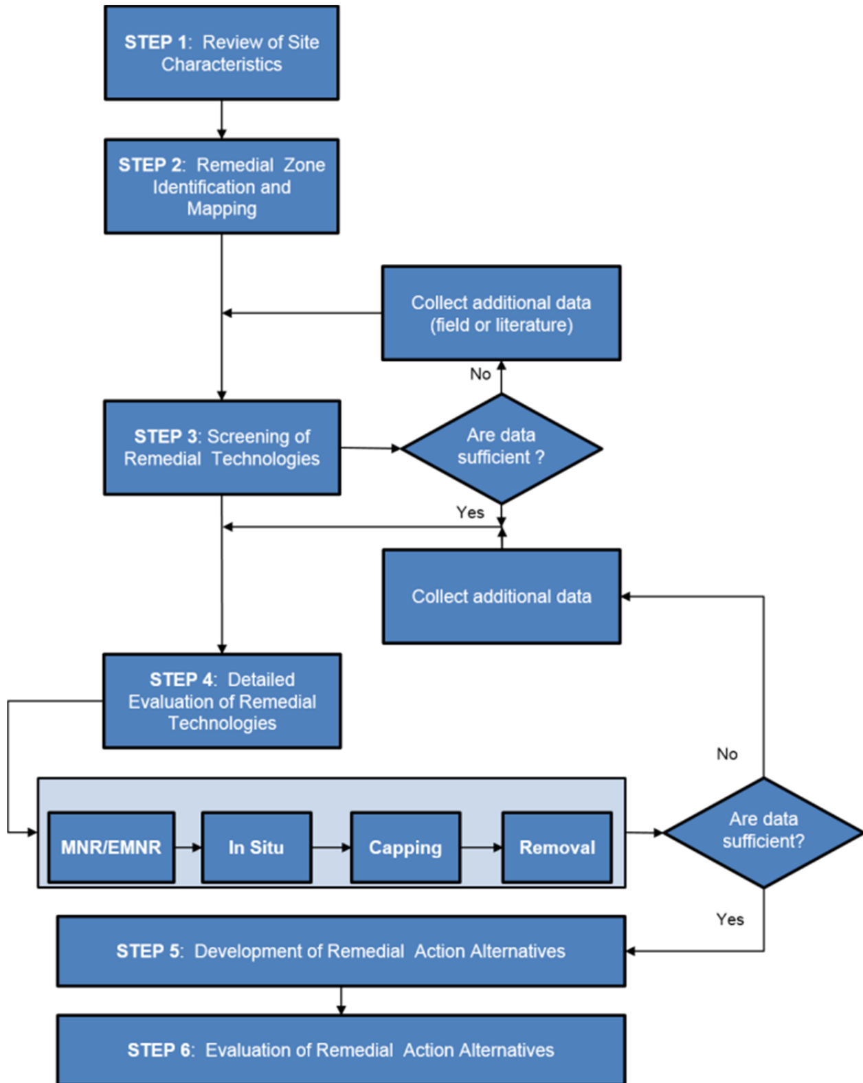
ITRC Remedy Selection for Contaminated Sediments ( http://www.itrcweb.org/cs-2/ ), Figure 2-1. Decision matrix flow chart
