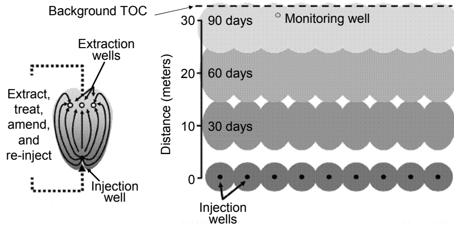
ITRC Technology Overview: In Situ Bioremediation of Chlorinated Ethene DNAPL Source Zones (BIODNAPL-1, 2005)
