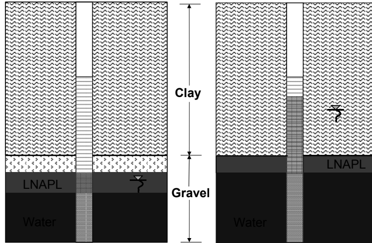
Monitoring well is a giant pore!
