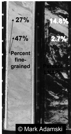
Soil texture | Fluorescing LNAPL
