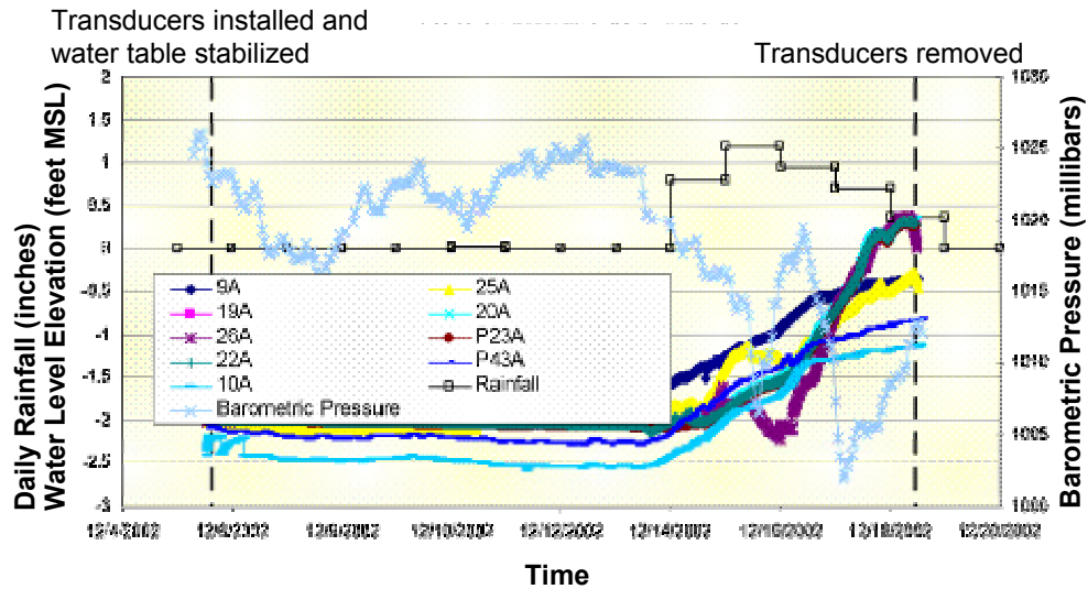
Change of Water Level Elevations with Time
