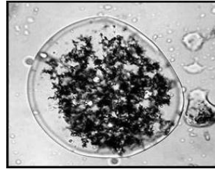
Micrograph of nanoscale iron within an emulsion droplet
