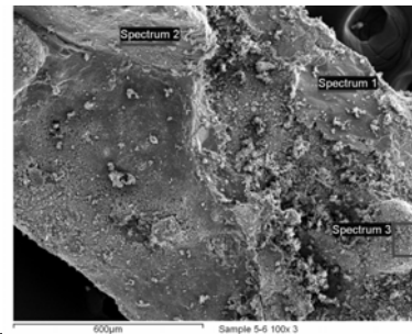
SEM image of hydrated iron, Hill AFB
