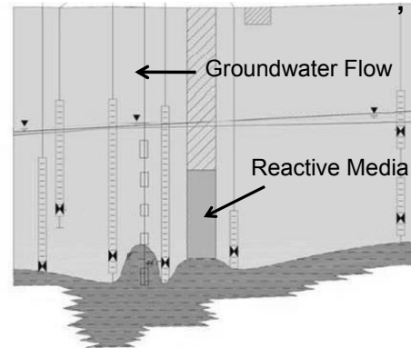
A ——— Cross Section ——— A
