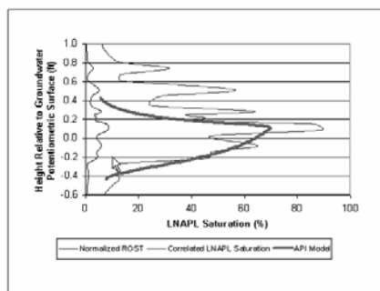
Figure 5 NAPL Saturation Log for NMS-09 (Gasoline-Like NAPL)
