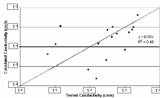
Figure 6 Comparison of Tested Versus Calculated NAPL Conductivities
