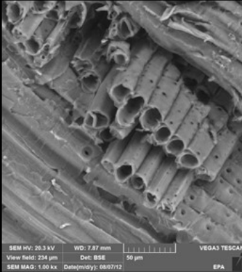
Raw Feedstock
