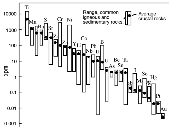
FIGURE 2.4—Average concentrations and ranges of trace elements in rocks. After Rose et al. (1979).
