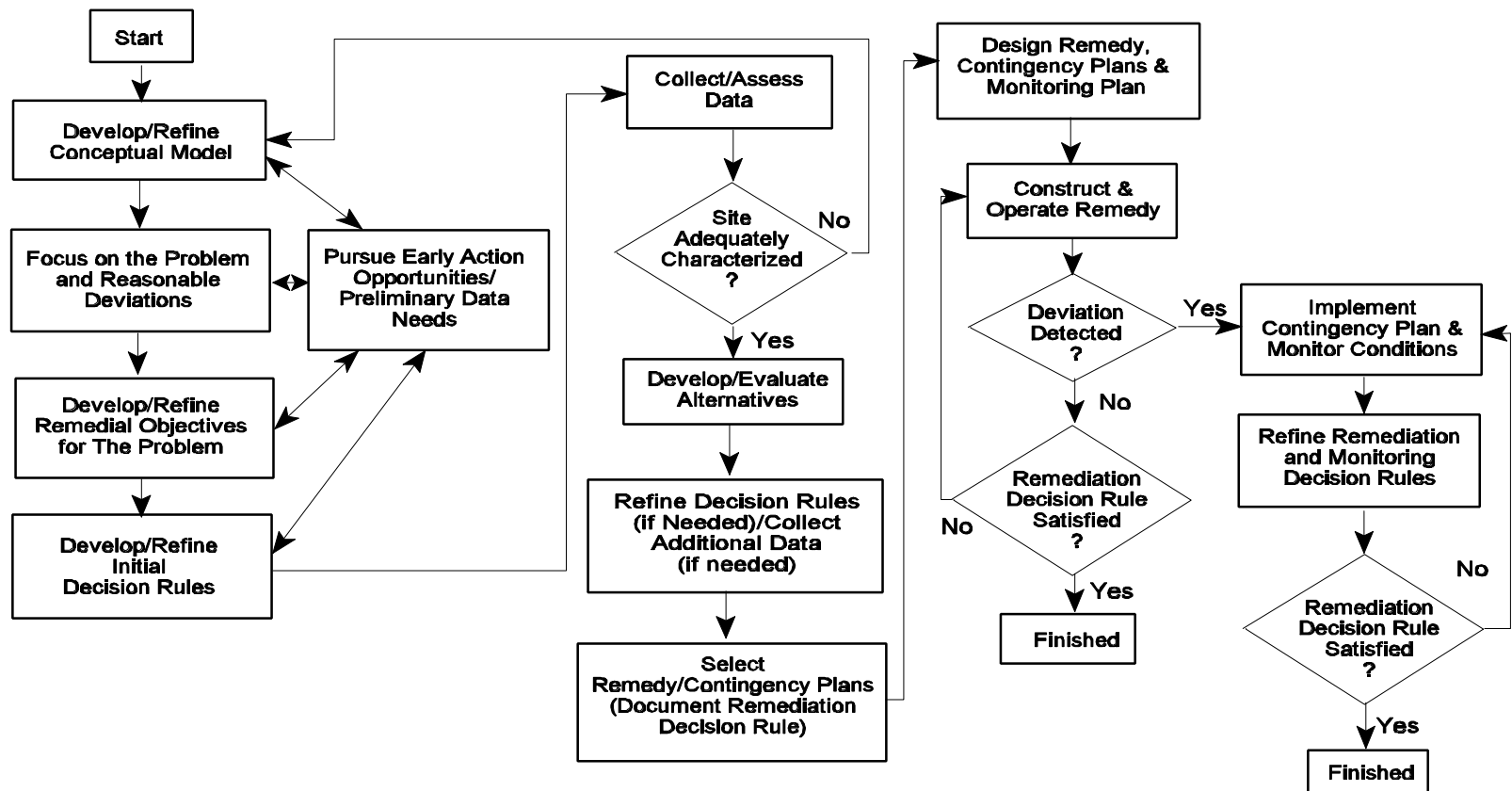
Figure A-1. DOE SAFER Framework Diagram
