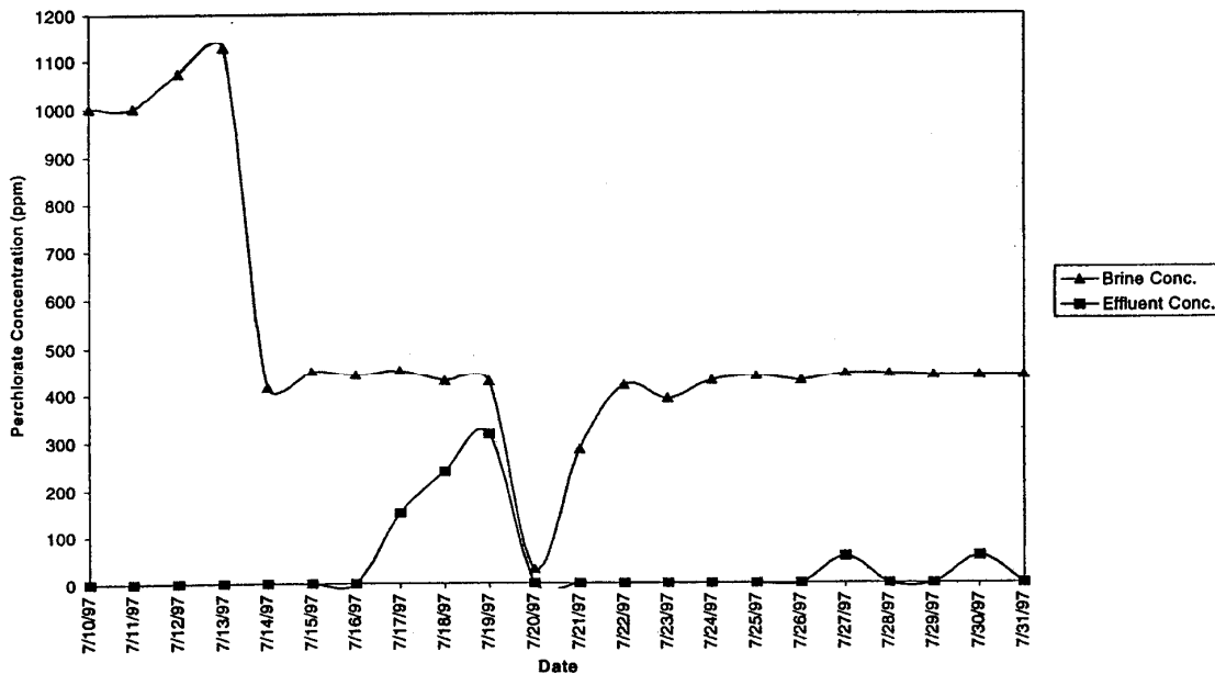
Figure 12. R-1400 Brine and Effluent Concentrations during Parallel Operation
