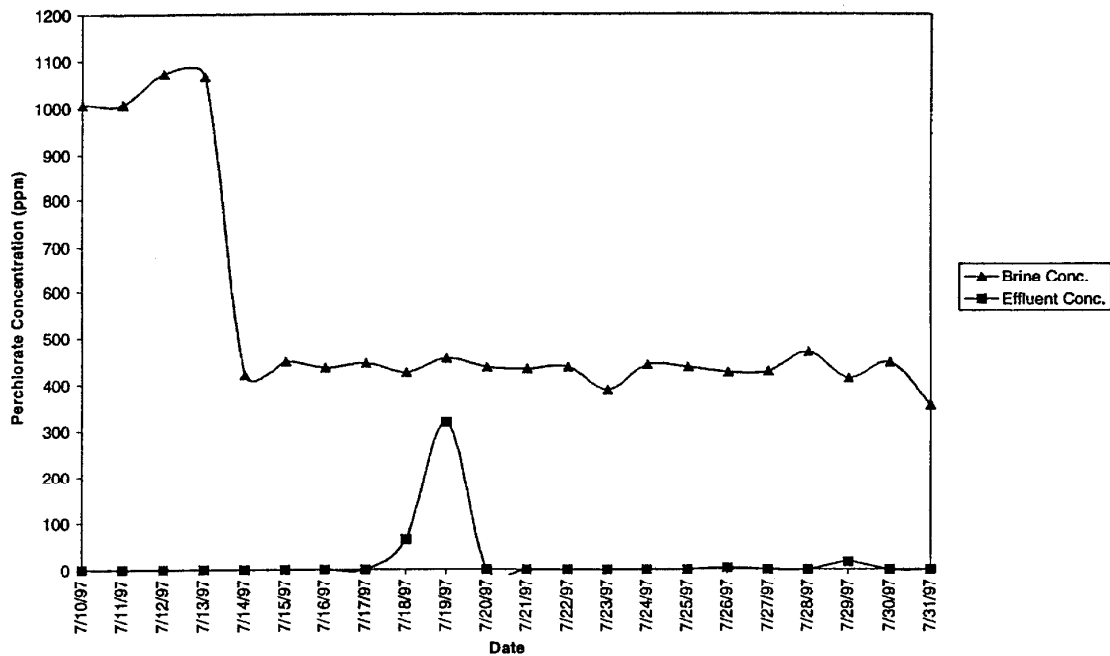
Figure 13. R-1700 Brine And Effluent Concentrations during Parallel Operation
