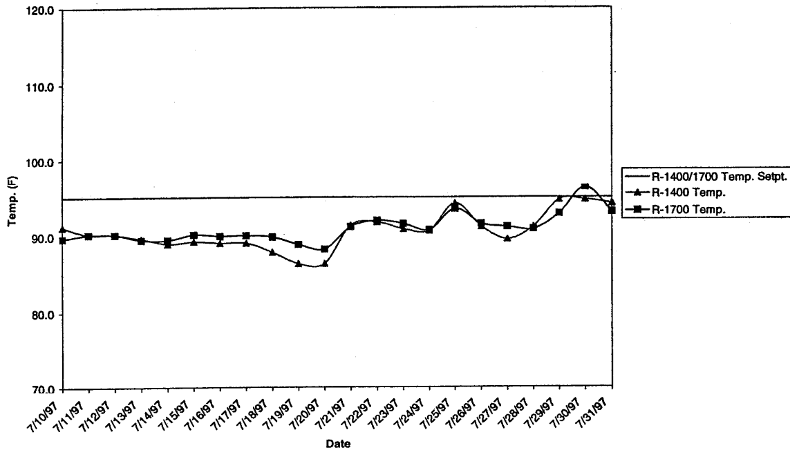
Figure 8. Reactor Temperature during Parallel Operation
