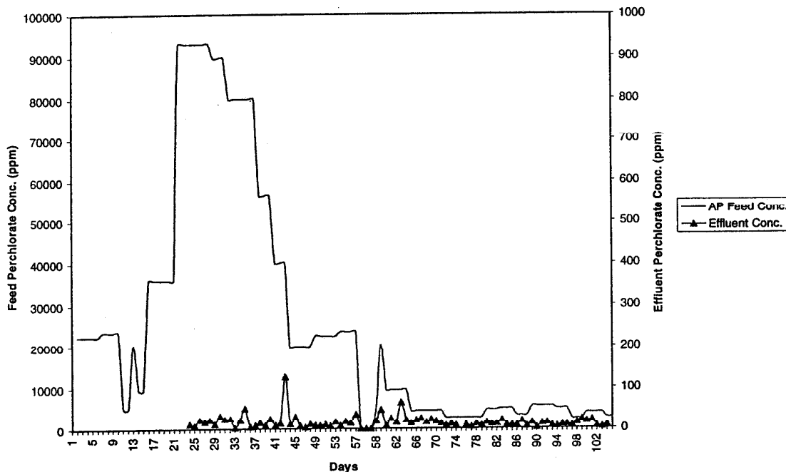
Figure 15. Thiokol AP Feed and Effluent Concentrations
