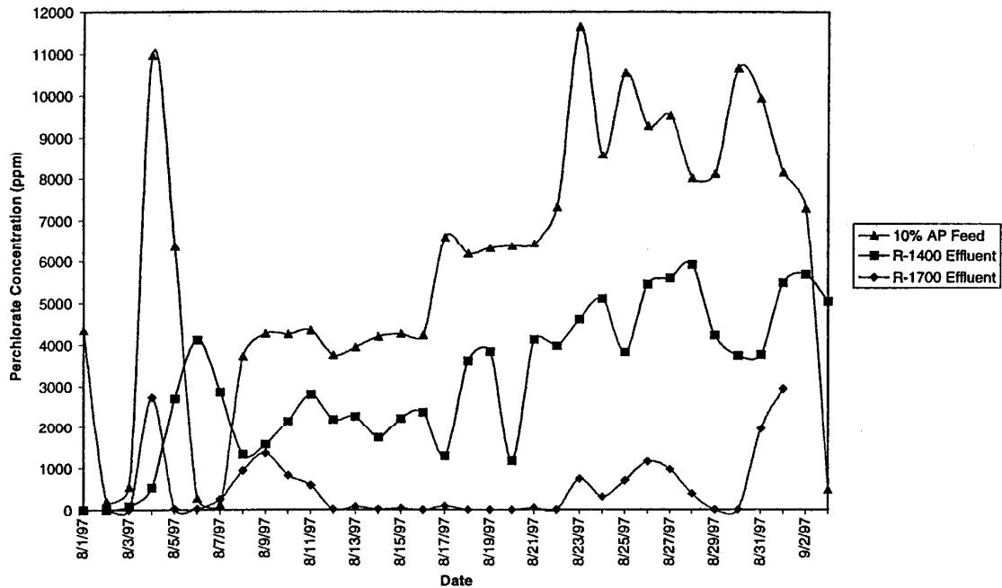
Figure 14. Series Operation: Calculated Perchlorate Feed Conc. vs. R-1400/1700 Concentrations
