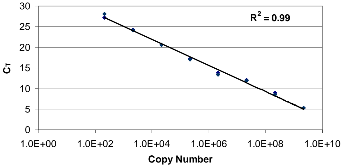
Figure 4.4. Standard Curve for the pcrA qPCR Assay. Purified plasmid containing the pcrA gene from Dechloromonas agitata was diluted for use as a copy number standard.
