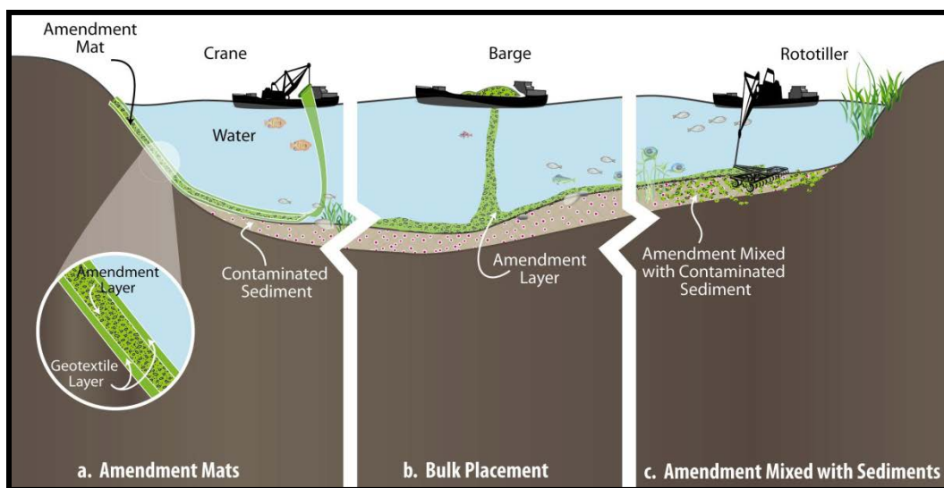
Figure 1: Placement Methods for Sediment Amendments
