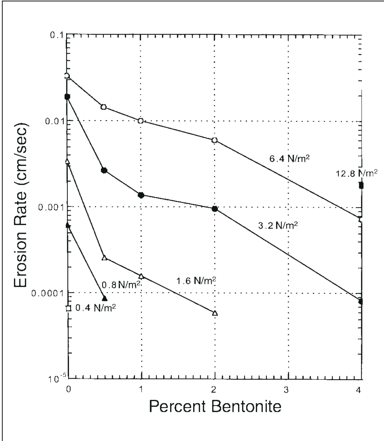
Figure 5. Erosion rates averaged for all densities as a function of percent bentonite added with shear stress (N/m 2 ). Note the difference in the vertical scale between Figures 5a, 5b, and 5c (Sheet 1 of 3)
