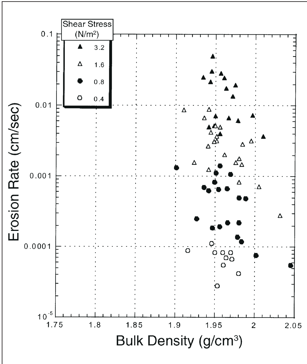
b. Erosion rates as a function of density, \rho^* , with shear stress ( N/m^2 ) as a parameter. Cap over base. Inset legend indicates values for different shear stresses
