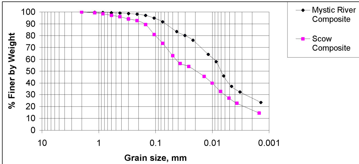
Figure 9. Cumulative grain size distribution (by weight) curves for pre- and post-dredged material samples after mechanical dredging
