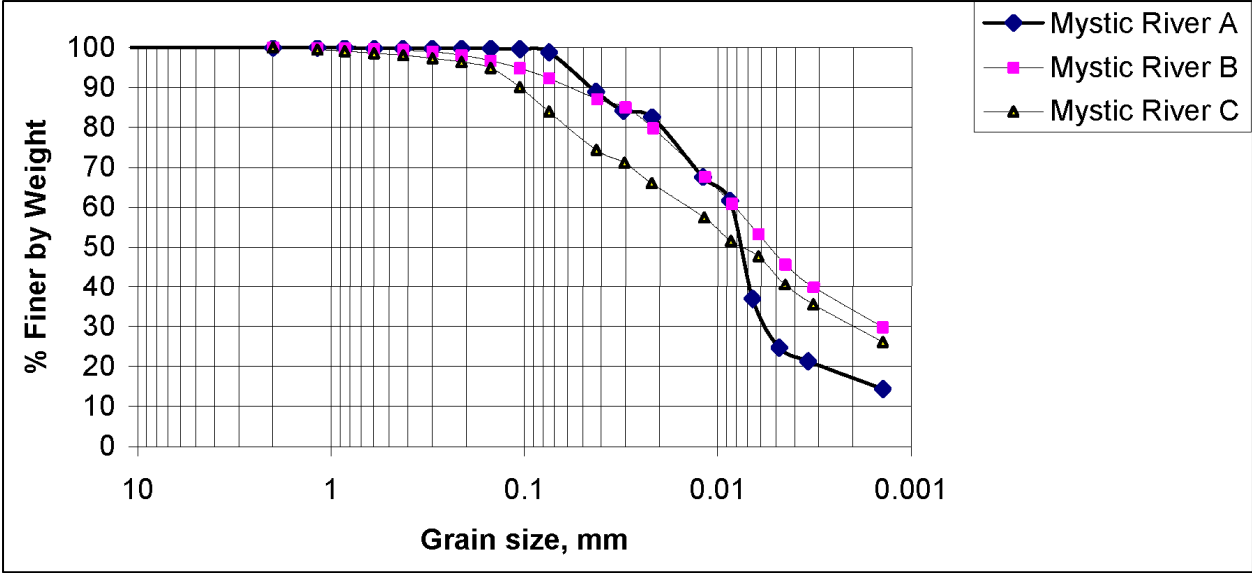
Figure 1. Cumulative grain size distribution (by weight) curves for river bottom samples
