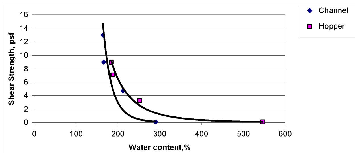
Figure 8. Comparison of pre-dredged and post-dredged vane shear strengths (to convert psf to kPa, multiply psf by 0.048)
