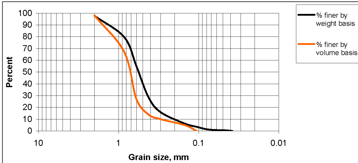
Figure 16. Variability between cumulative grain size distributions (weight vs. volume basis) for identical materials
