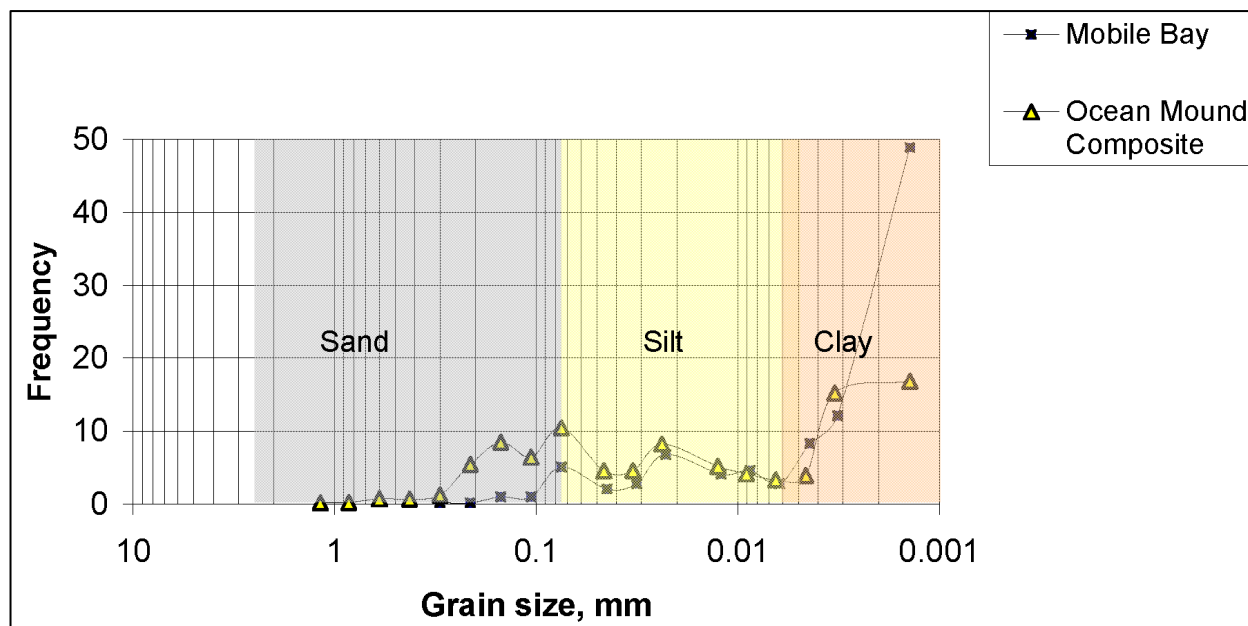
Figure 10. Frequency grain size distribution (by weight) curves for pre-dredged and post-placed material samples
