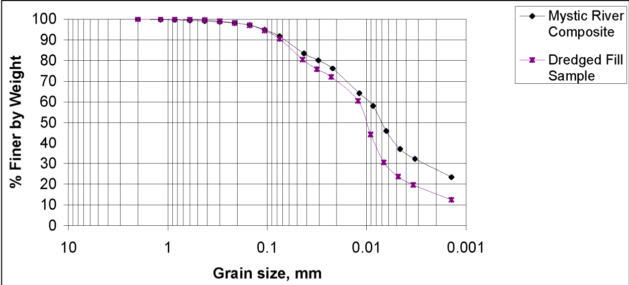
Figure 11. Cumulative grain size distribution (by weight) curves for pre-dredged and post-placed material samples after mechanical dredging and dump scow placement
