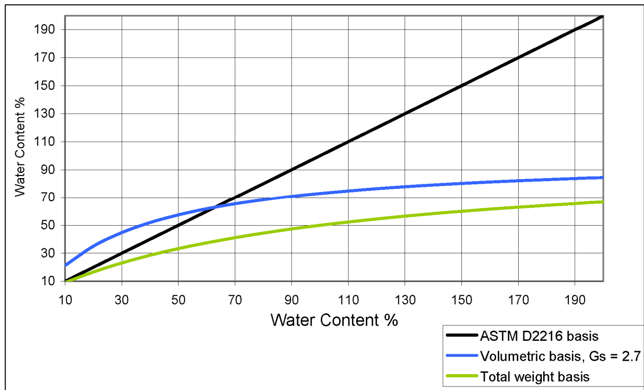
Figure 15. Comparison of water content definitions
