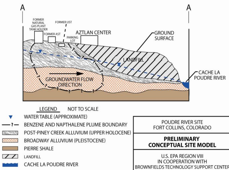
Figure 2: Preliminary CSM Representation. This Preliminary CSM summarizes general site information, including primary site attributes, geologic stratigraphy, groundwater potentiometric surface and flow direction, groundwater-surface water relationship, and presumed extent of soil and groundwater contamination. This form of CSM can be an effective method of communicating site conditions to a diverse audience in an easy-to-understand format.
