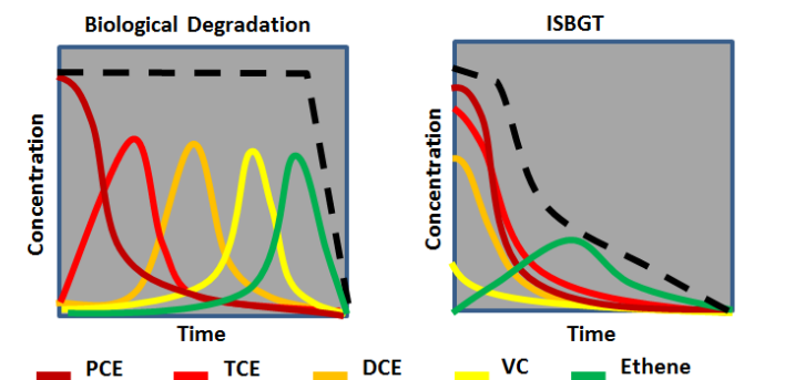
Figure 3. Biological vs. ISBGT Pattern of Degradation (Courtesy of Battelle)
