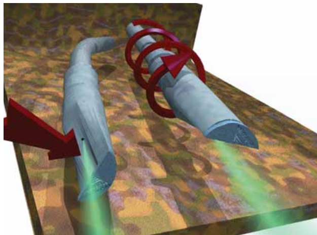
Exhibit A-13. Steering The Borehole
