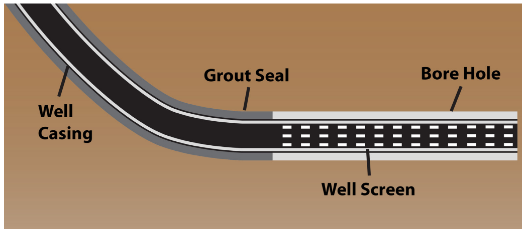
Exhibit A-26. Schematic Of Horizontal Well Construction
