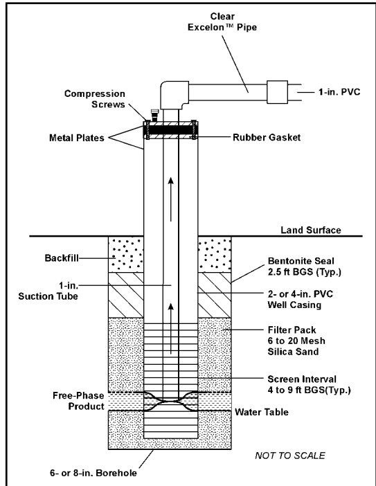
Figure 3. Diagram of Extraction Well
