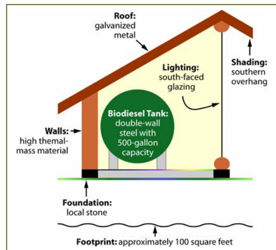
Figure 3. Green construction techniques can be integrated into BMPs for small structures used to store field equipment or to house treatment components such as pump equipment.
