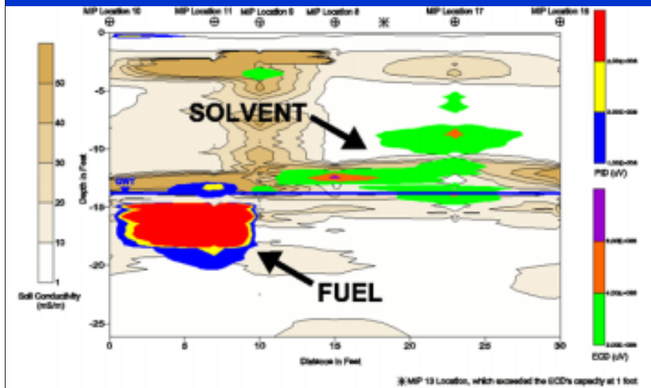
Figure 1 PID & ECD Response Threshold Dry Cleaner Site January 30-31, 2001, February 1, 2001
