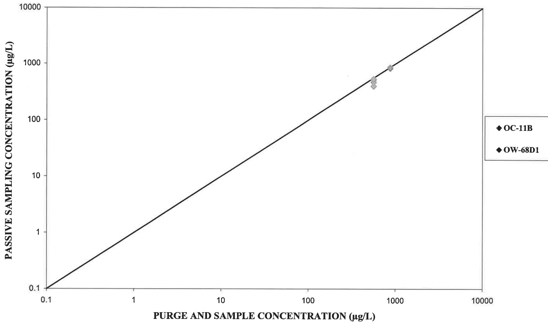
FIGURE 3-14 COMPARISON OF METHYLENE CHLORIDE CONCENTRATIONS
