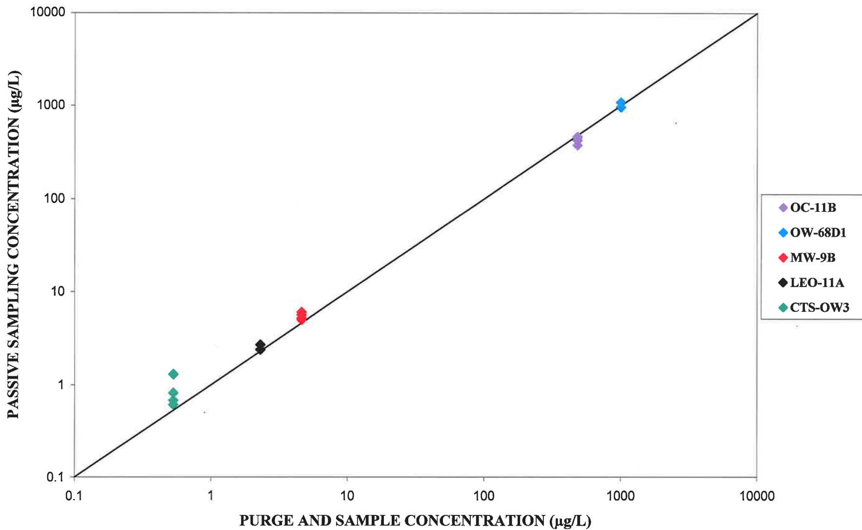
FIGURE 3-12 COMPARISON OF CHLOROFORM CONCENTRATIONS
