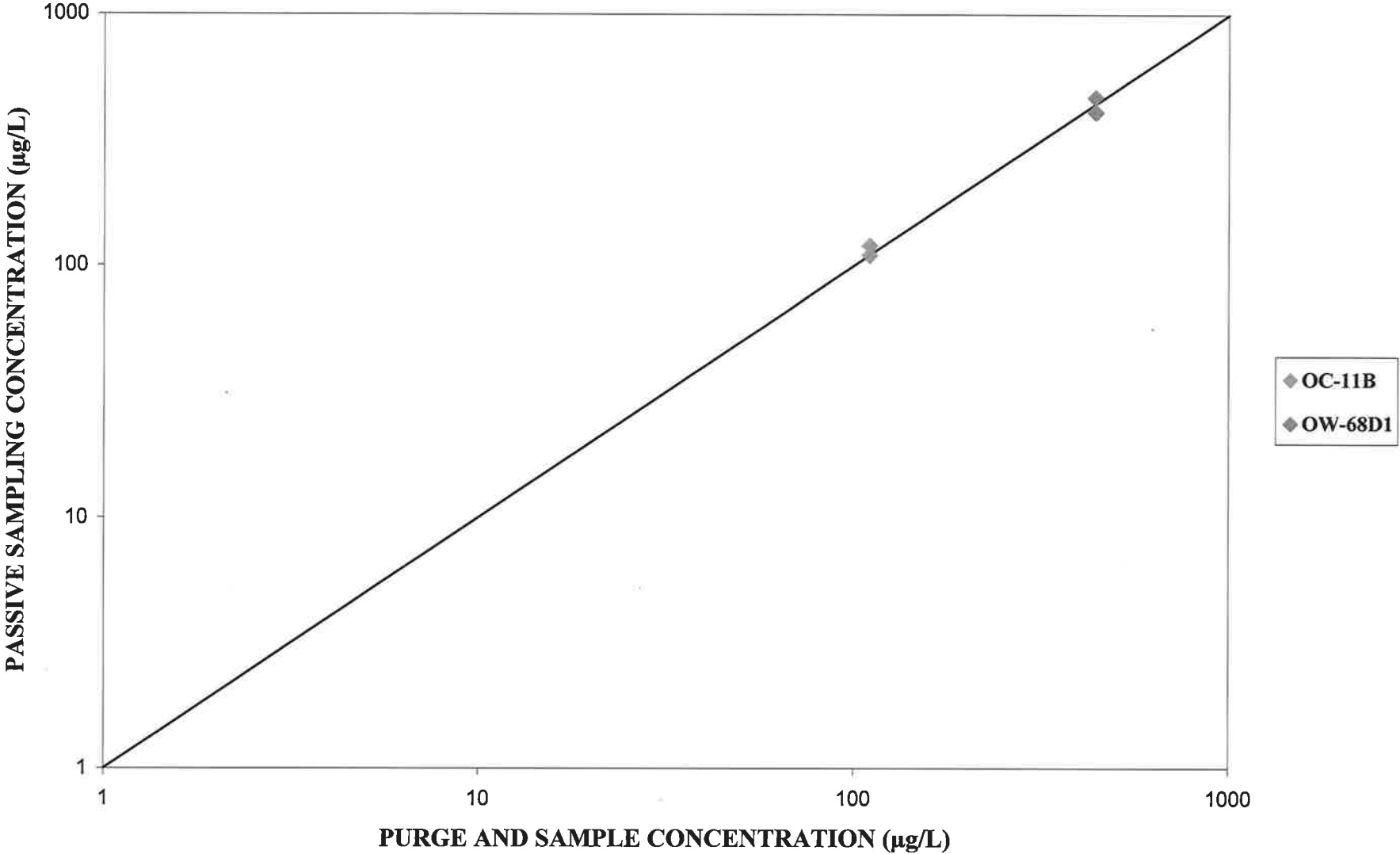
FIGURE 3-10 COMPARISON OF PCE CONCENTRATIONS
