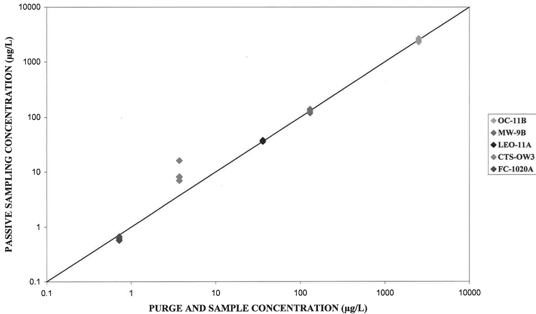
FIGURE 3-11 COMPARISON OF TCE CONCENTRATIONS
