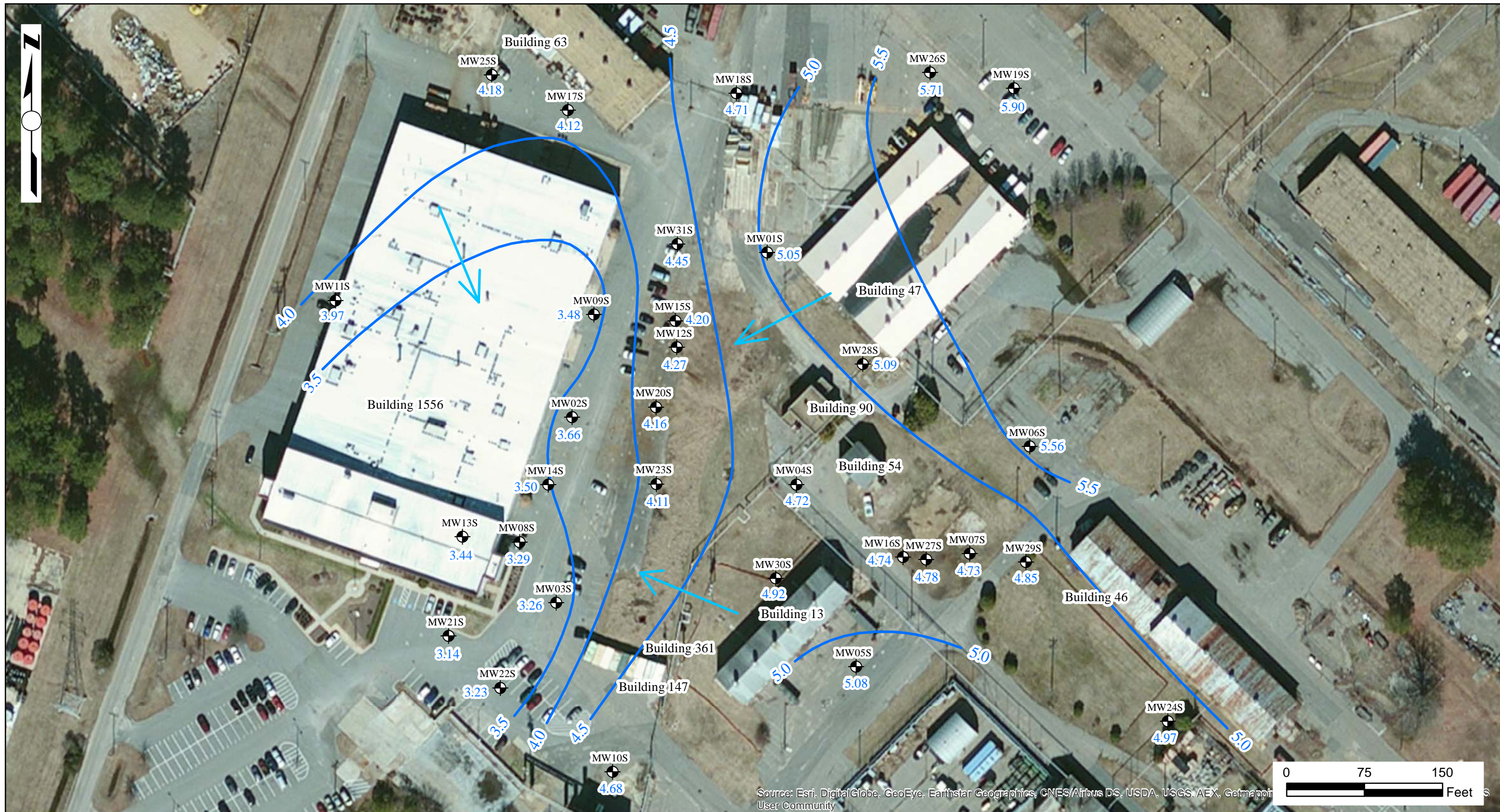
FIGURE 2 : Groundwater Potentiometric Surface Contours November 2015
