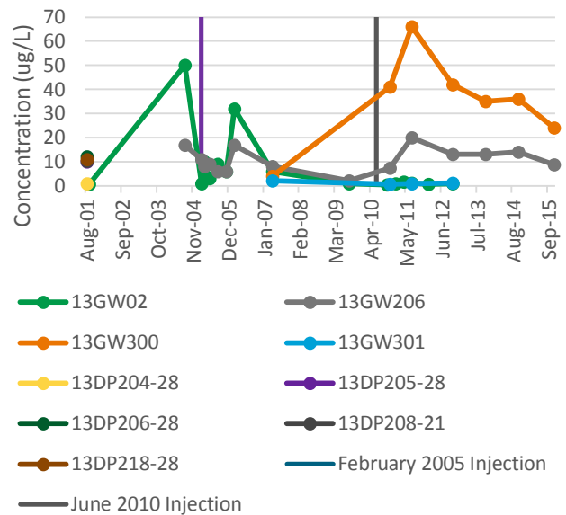
Chart WO-6 VC - On-site Wells NSWC White Oak Site 13
