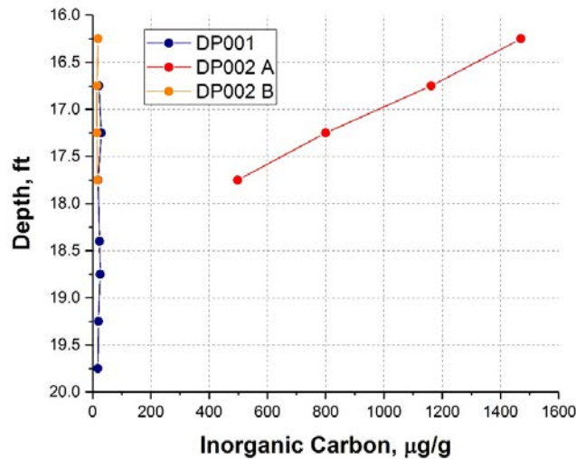
Figure 5-24. Inorganic Carbon vs. Depth in Former St. Louis Ordnance Plant OU1 in ZVI Core Samples
