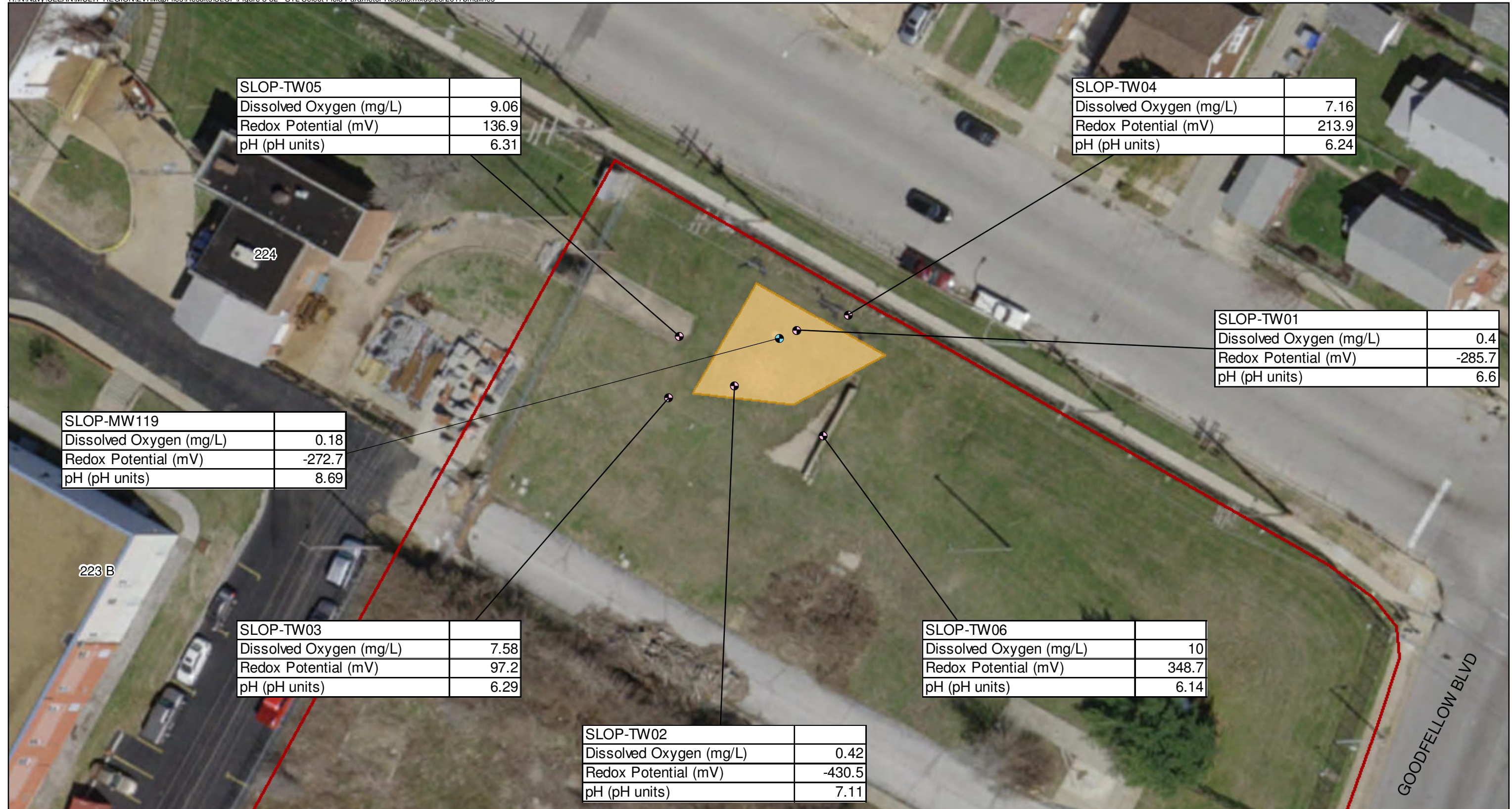
Figure 5-10 Select Field Parameter Results - January 2017 Former St. Louis Ordnance Plant OU1 St. Louis, Missouri
