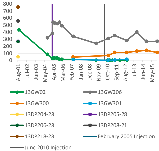
Chart WO-6 VC - On-site Wells NSWC White Oak Site 13
