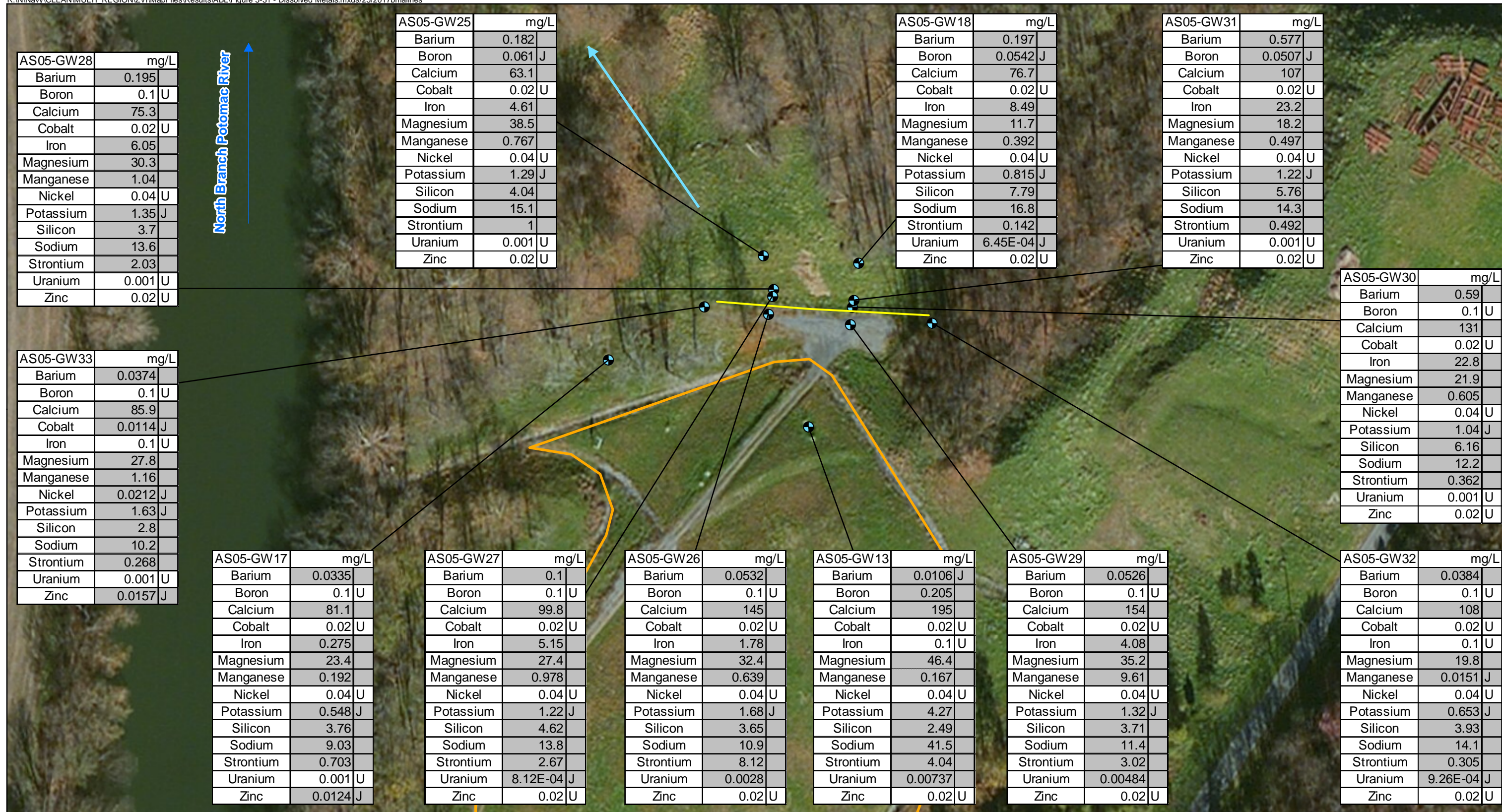
Figure 5-9 Dissolved Metals - January 2017 Allegany Ballistics Laboratory Site 5 Rocket Center, WV
