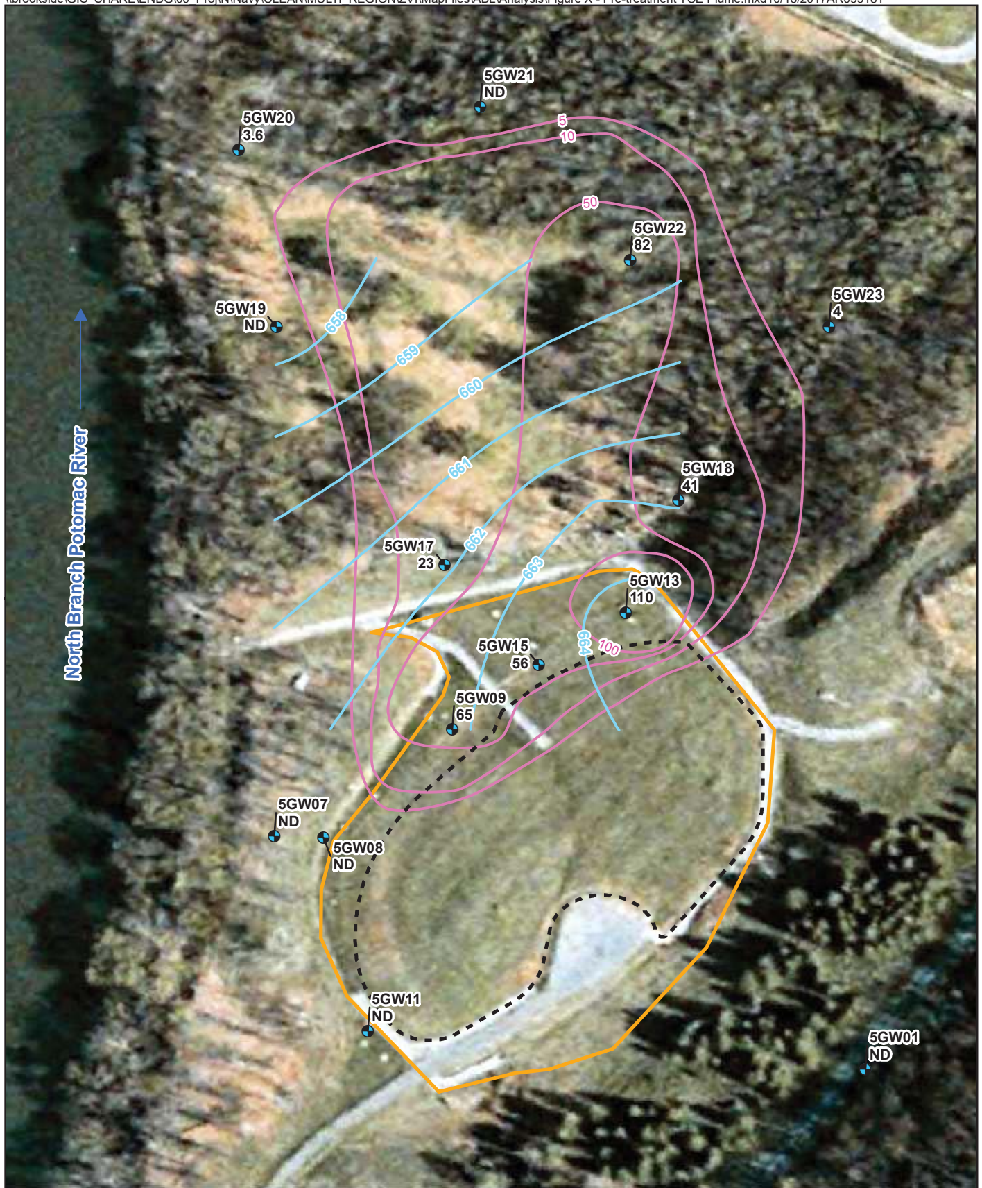
Figure 4-3 Pre-treatment TCE Plume Allegany Ballistics Laboratory Rocket Center, West Virginia
