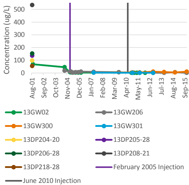
Chart WO-5 trans-1,2-DCE - On-site Wells NSWC White Oak Site 13
