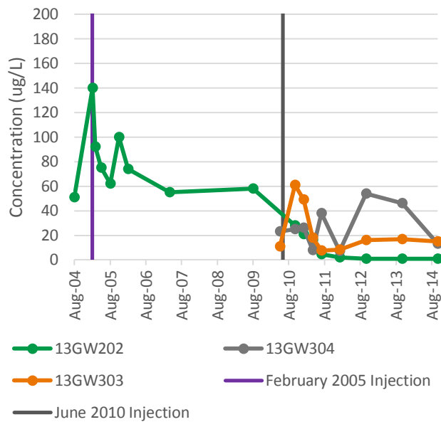
Chart WO-19 trans-1,2-DCE - Off-site Wells NSWC White Oak Site 13
