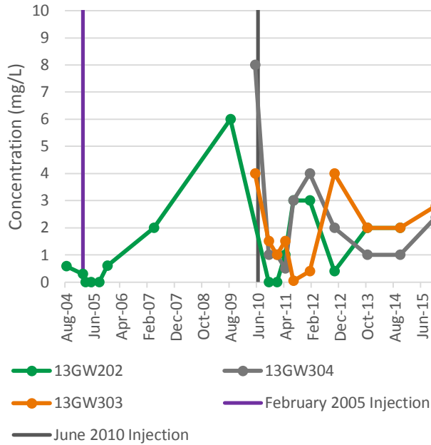
Chart WO-21 DO - Off-site Wells NSWC White Oak Site 13
