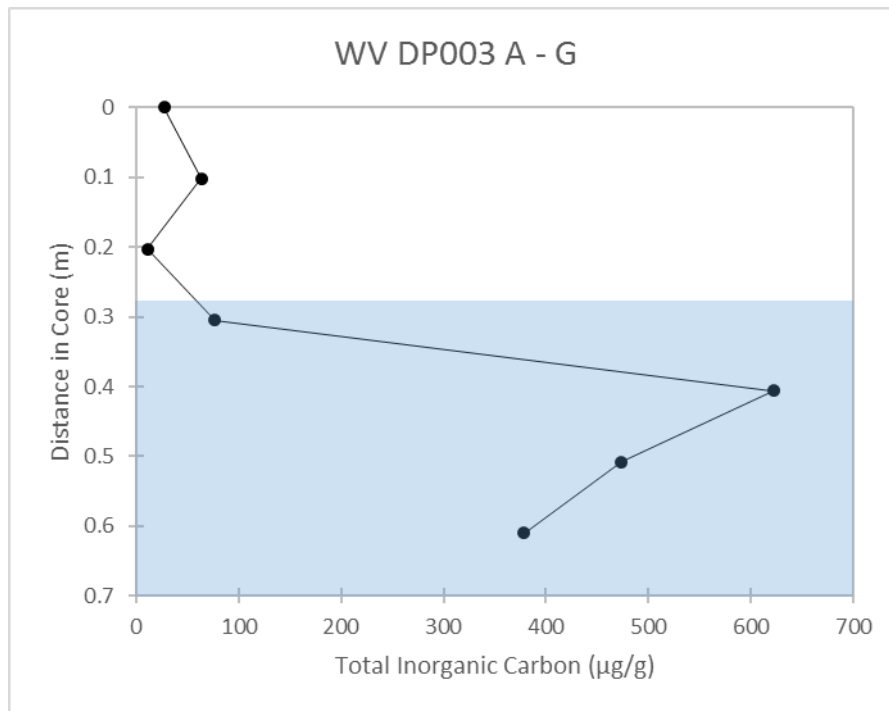
Figure 5-16. Inorganic Carbon Concentrations in ABL Site 5 Core DP003 The blue-shaded region represents core material dominated by granular iron.
