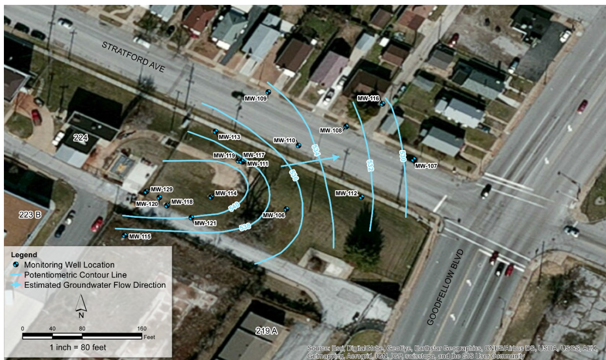
Figure 4-6. Former St. Louis Ordnance Plant OU1 Groundwater Contour Map (April 2015)
