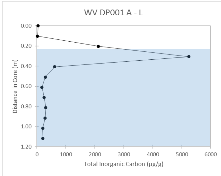
Figure 5-15. Inorganic Carbon Concentrations in ABL Site 5 Core DP001 The interface region shows an abrupt increase in the concentration of solid-phase carbonate; the blue-shaded region represents core material dominated by granular iron.
