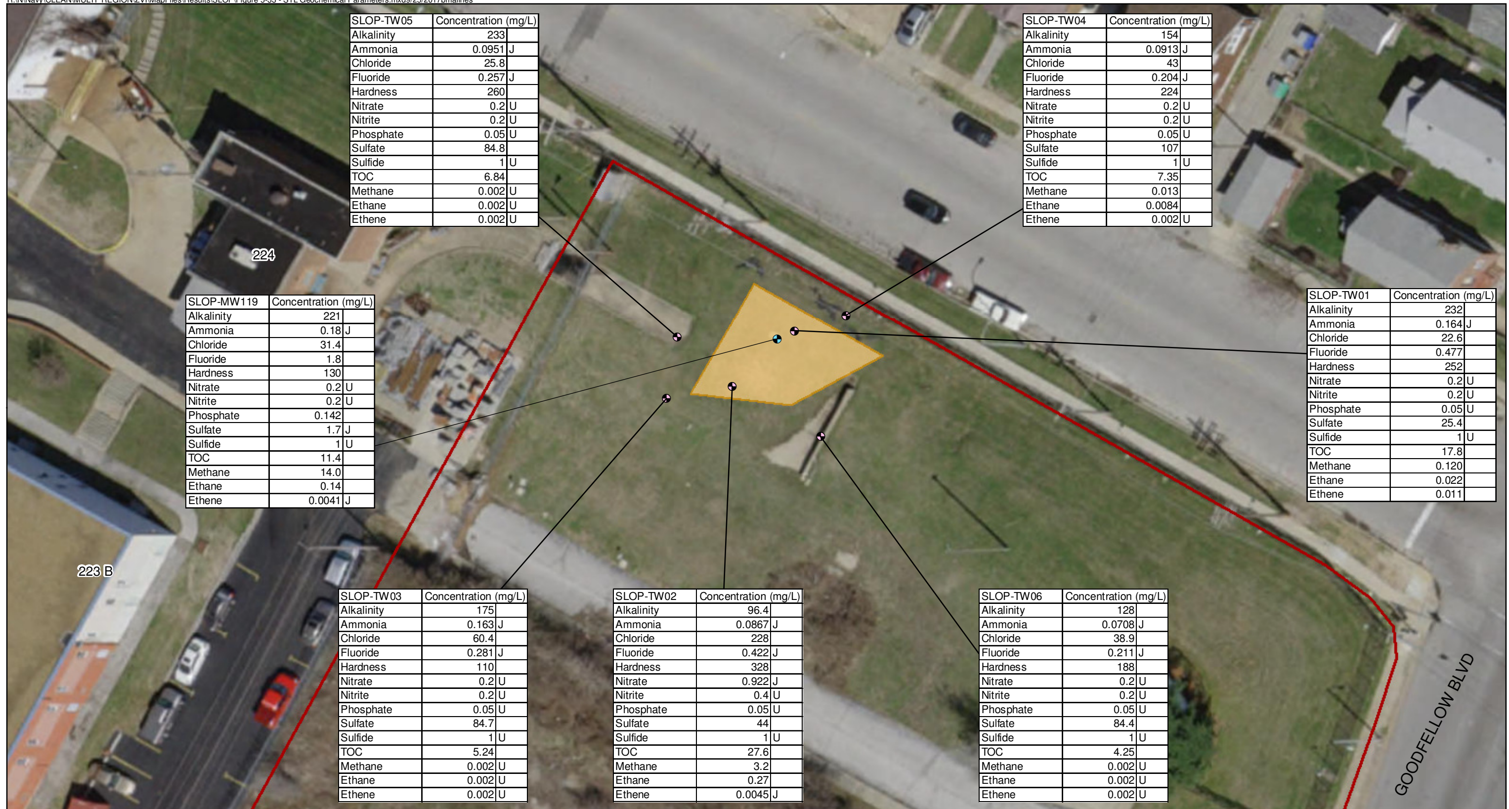
Figure 5-11 Geochemical Parameters - January 2017 Former St. Louis Ordnance Plant OU1 St. Louis, Missouri
