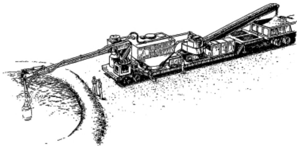
Figure 6-7. Schematic of a trailer-mounted mobile mixing plant (Courtesy Beardsley & Piper).
