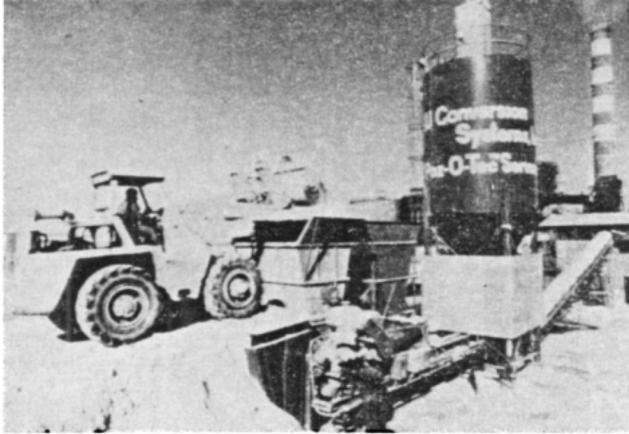
Figure 6-13. Large modular mixing plant (Courtesy IU Conversion).
