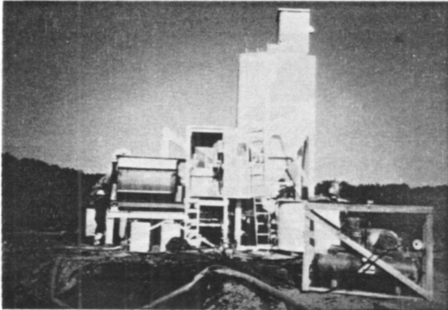
Figure 6-12. Small modular mixing plant (Courtesy Solid Tek).
