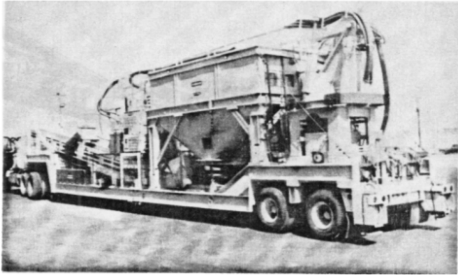
Figure 6-9. Open mobile mixing plant (Courtesy Beardsley & Piper).
