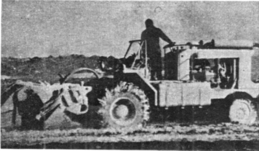
Figure 6-18. Mixing waste materials with stabilization/solidification reagents in area mixing (Courtesy Soil Recovery).
