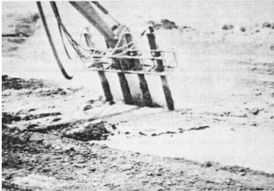
Figure 6-4. In-situ mixing by direct reagent injection (Courtesy ENRECO, Inc.).
