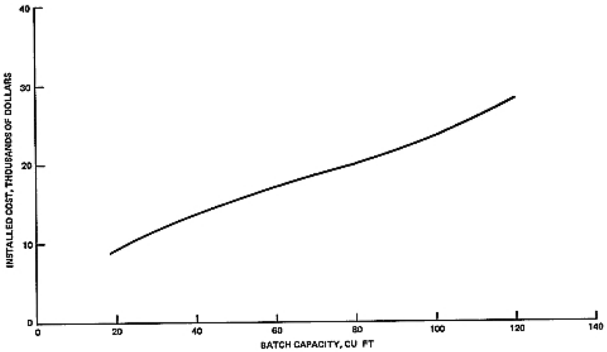
Figure B-18. Installed cost for ribbon blenders.
