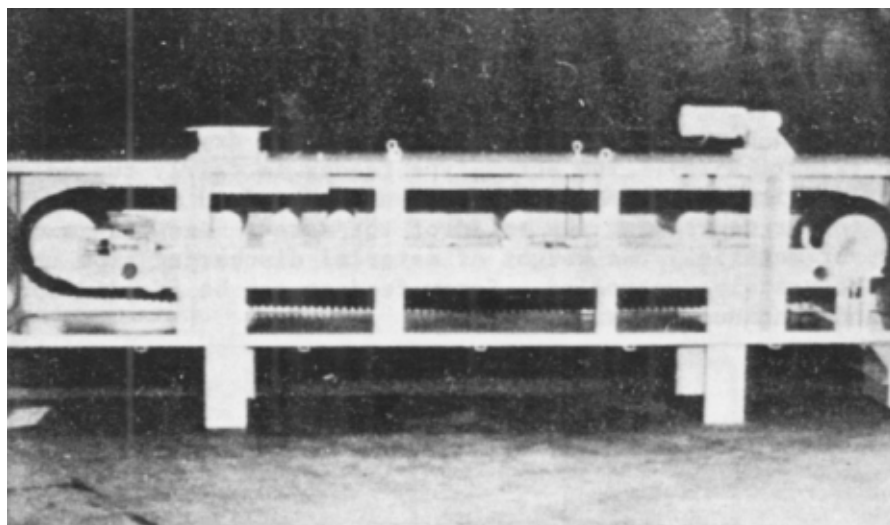
Figure B-26. Typical weigh feeder system (Courtesy Rexnord).
