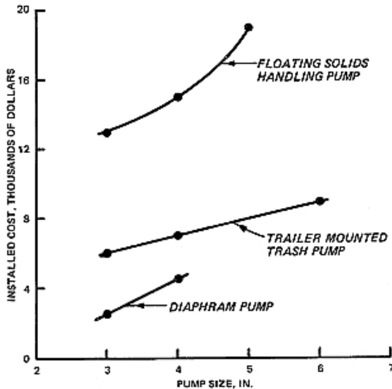
Figure B-5. Typical costs for pumping systems.
