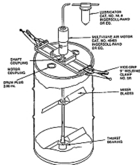
Figure 6-2. Typical spill cleanup system (Courtesy Delaware Custom Materials).
