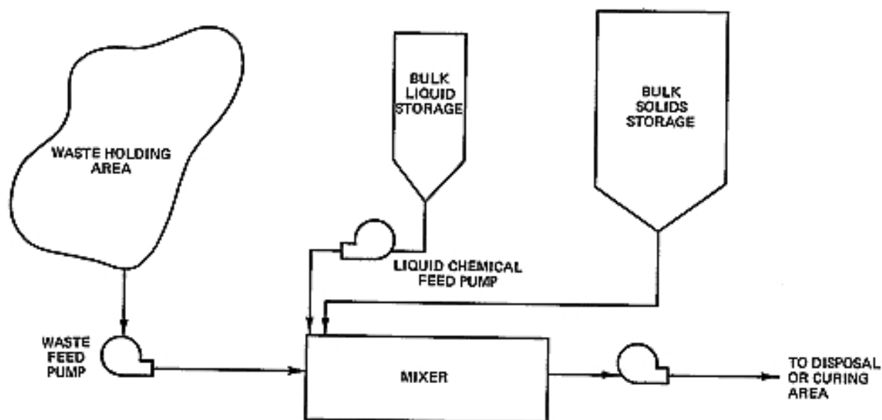
Figure 6-6. Schematic of plant mixing scenario.
