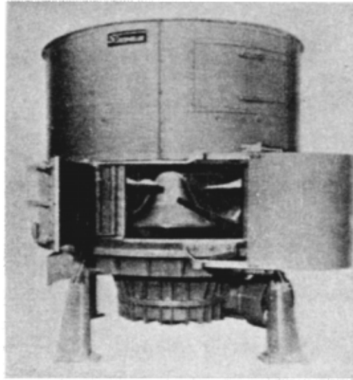
Figure B-19. Typical muller mixer (Courtesy Beardsley & Piper).
