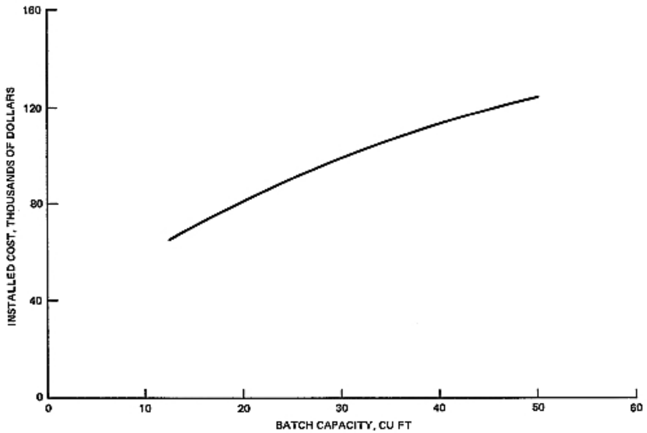
Figure B-20. Installed cost for muller mixers.
