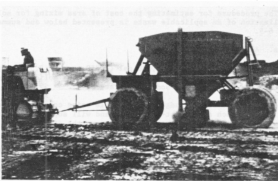
Figure 6-17. Adding stabilization/solidification reagent for area mixing (Courtesy Soil Recovery).
