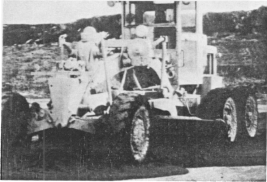
Figure 6-16. Spreading untreated material for area mixing (Courtesy Soil Recovery).
