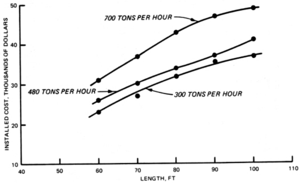
Figure B-8. Installed portable conveyor system costs.
