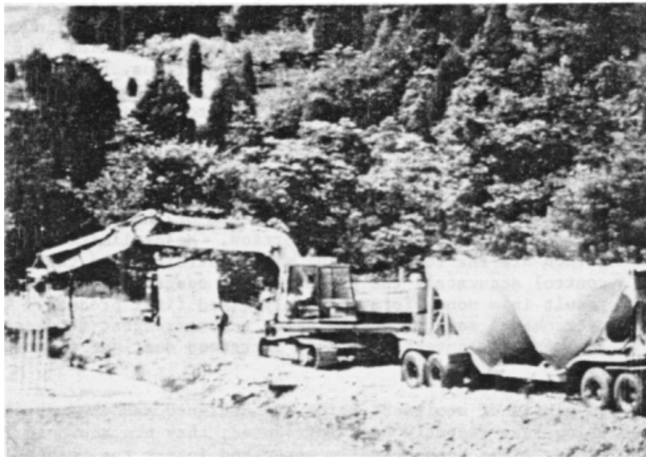
Figure 6-5. In-situ mixing equipment (Courtesy American Resources Corporation).
