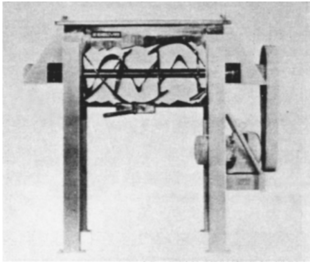
Figure B-17. Typical ribbon blender (Courtesy Beardsley & Piper).
