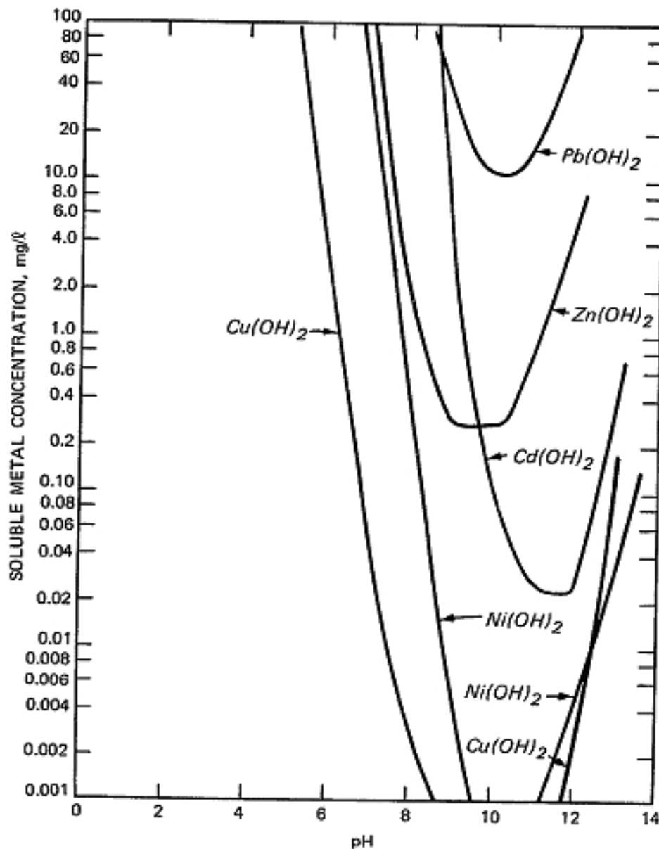
Figure 2-2. Theoretical solubilities of selected amphoteric metal hydroxides.
