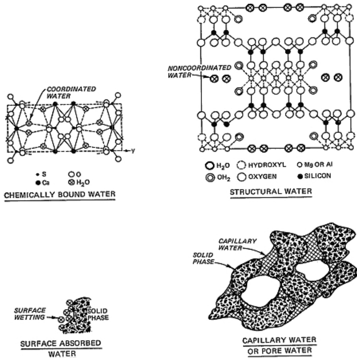
Figure 2-1. Mechanisms retaining water and ionic materials on and in solid phases.
