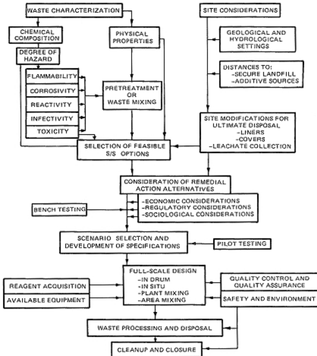
Figure 1-1. Flow chart for evaluating the stabilization/solidification (S/S) option.
