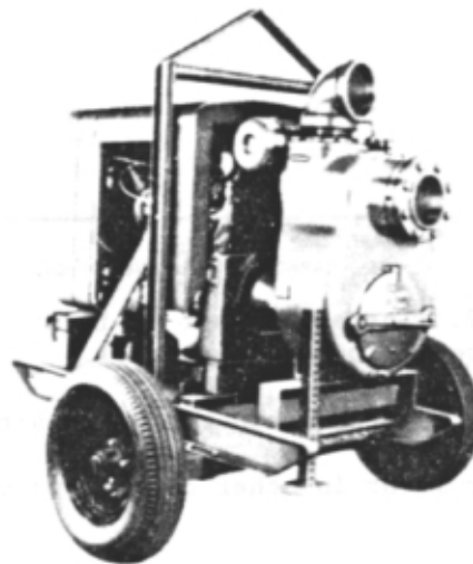
Figure B-3. Trailer-mounted centrifugal pump (Courtesy Gorman Rupp Company).
