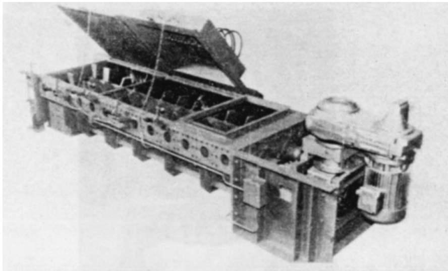
Figure B-21. Typical twin-shaft rotor mixer (Courtesy Beardsley & Piper).
