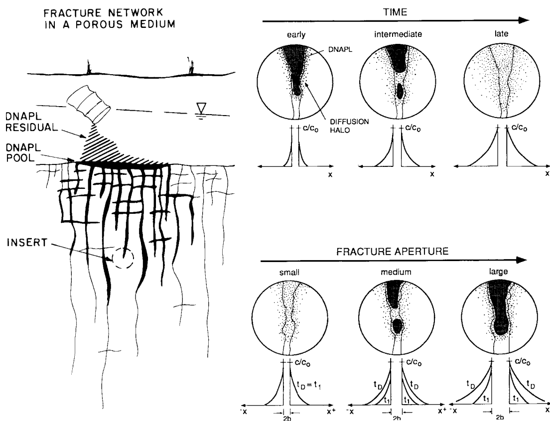
Conceptualization of DNAPL persistence and distribution with DNAPL mass loss due to diffusion in water-saturated fractures in a porous medium (such as a fractured clay till or sedimentary rock) as a function of: a) time; and b) fracture size (aperture). Diffusion halos around fractures containing DNAPL become large (more developed) with increases in time, as shown with the concentration vs. distance plots for the three relative time periods in part a. At any particular time t_1 , the DNAPL mass distribution will vary in different size fractures, with DNAPL disappearance occurring most rapidly in the smallest fractures; residual or disconnected DNAPL will be present in medium-sized fractures, and free DNAPL will be present in the largest fractures that are connected to overlying DNAPL pools. DNAPL disappearance times ( t_D ) increase with an increase with fracture aperture.
