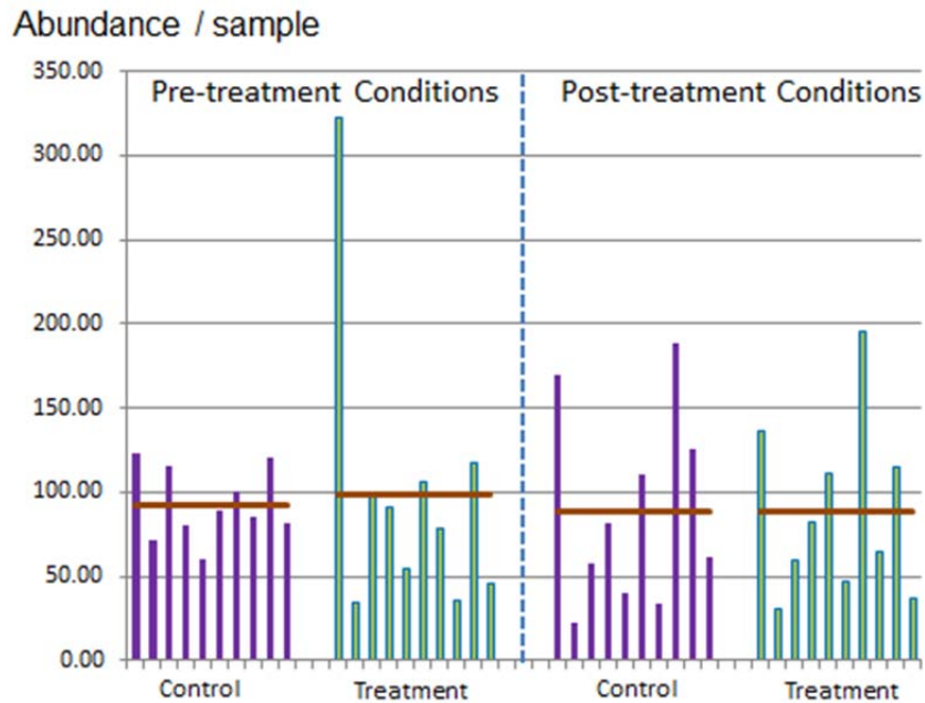
Figure 42. Abundance of benthic invertebrates in control and treatment plots of LCC prior to treatment (September 2009) and 10 months post-treatment (October 2011). Averages are indicated by horizontal bars.
