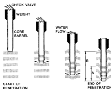
FIG. 1 Deformations Caused by Open-Barrel Core Samplers (1) 1
