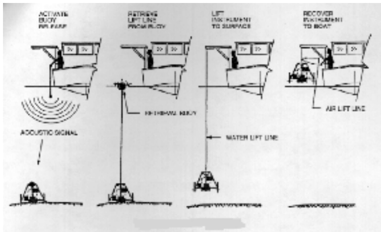
Figure 4. BFS2 Retrieval
