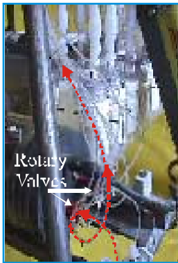
Rotary Sample Valves, tubing and sample bottles (Sample route highlighted)
