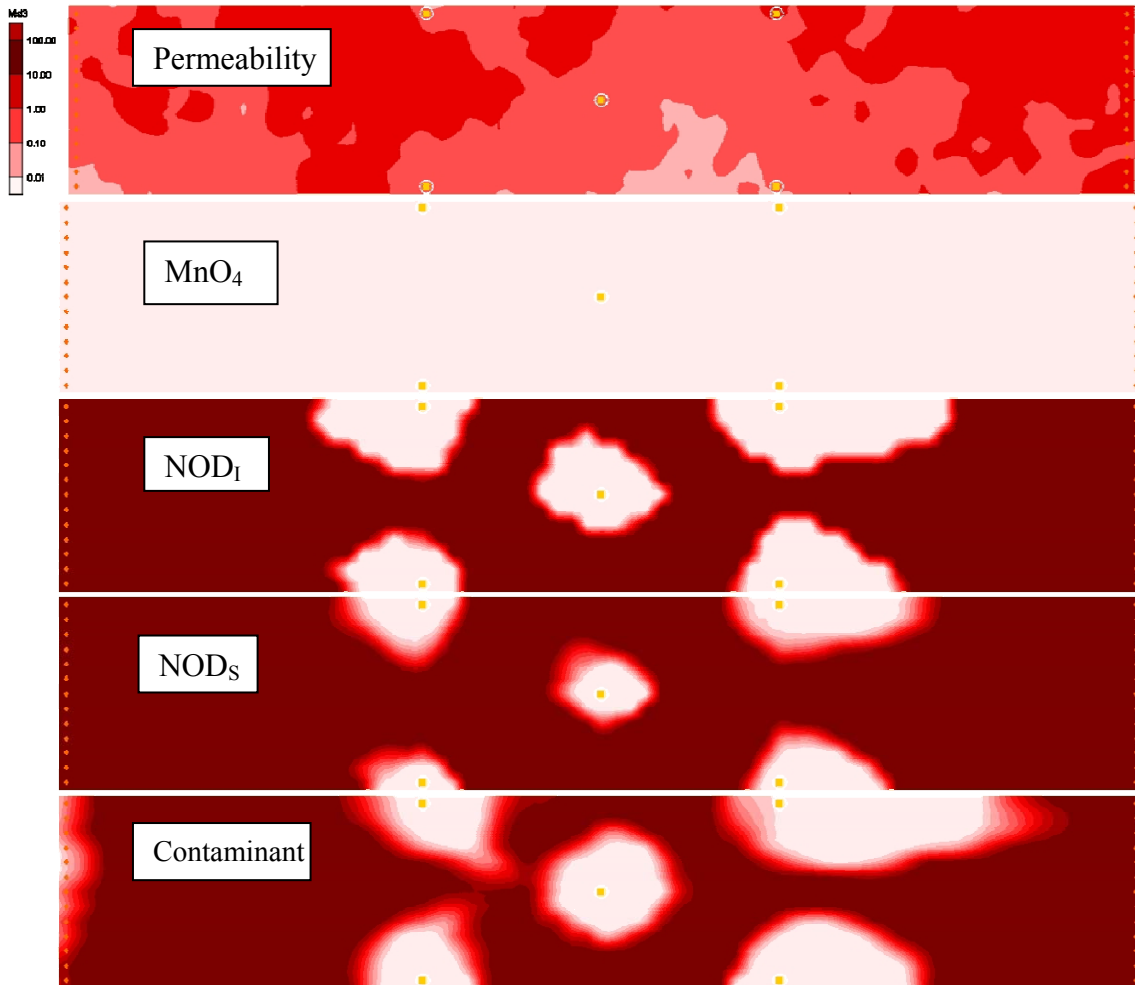
Figure 5.3: Horizontal Hydraulic Conductivity, MnO_4 , NOD_1 , NOD_s and Contaminant Distributions in Top Layer of Aquifer (see Figure 5.4) at 120 days after Injection for Moderately Heterogeneous Aquifer (realization #3) when Wells 1-5 are Injected with SF_V = SF_M = 0.25 . Deep red indicates a very high concentration or value, white indicates very low or zero.
