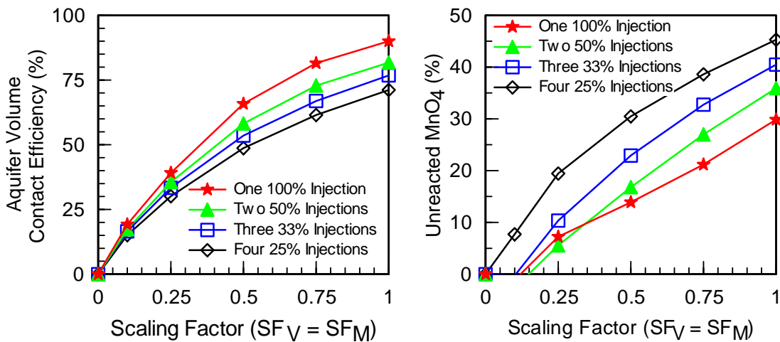
Figure 5.8: Effect of Reinjection on E_V and U at 180 days for SF_V = SF_M in a Medium Heterogeneity Aquifer. Well spacing = 3 m.
