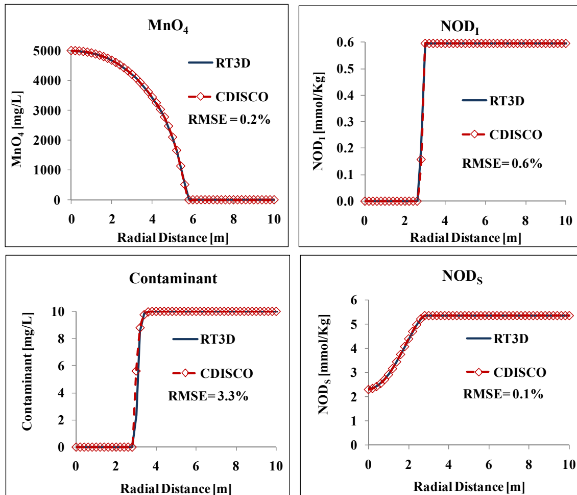
Figure 6.2: Comparison of CDISCO and RT3D Simulations of MnO_4 , NOD_I , NOD_S and Contaminant Concentration at 10 days after Injection for \alpha_L = 0.1 m.
