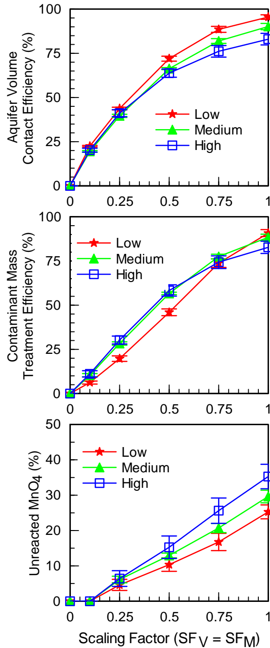
Figure 5.11 Effect of Low, Medium and High Aquifer Heterogeneity on E_V , E_M and U at 180 days ( SF_V = SF_M ) (error bars show the standard deviation observed in five permeability realizations for each level of heterogeneity)
