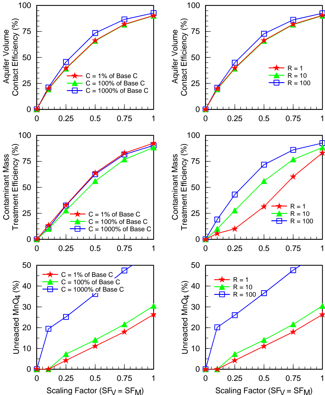
Figure 5.10: Effect of Initial Contaminant Concentration (a) and Contaminant Retardation Factor (b) on E_V , E_M , and U at 180 days for SF_V = SF_M .
