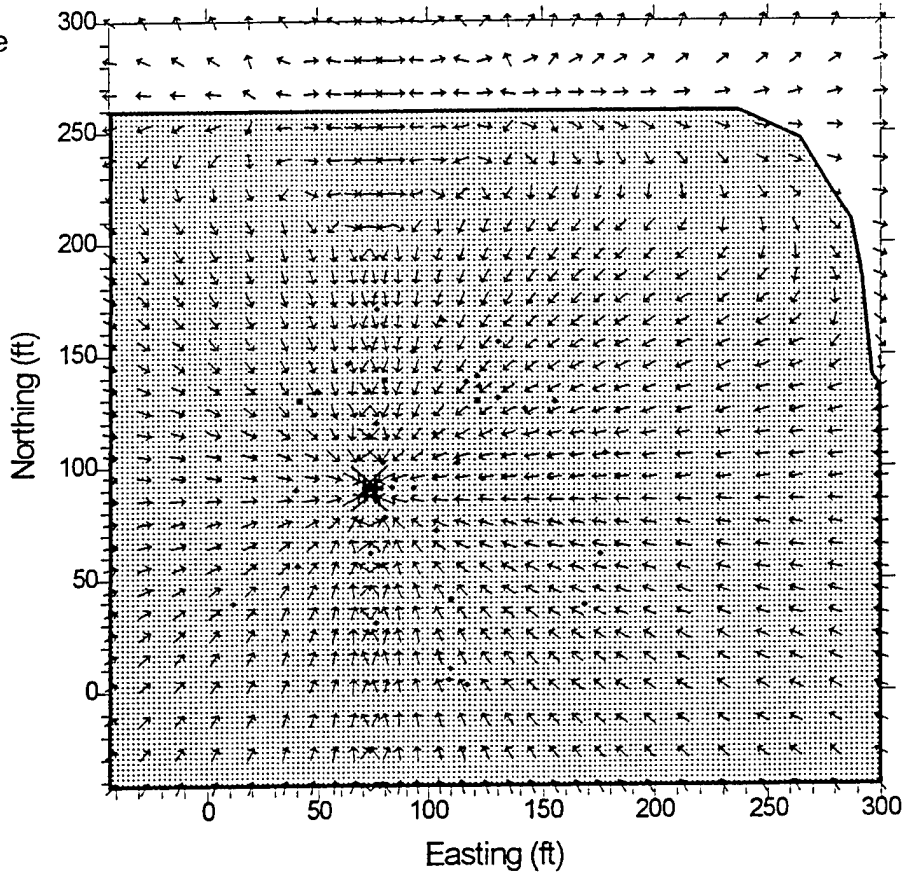
Figure 3-12B. Simulated Flow Vectors for the Air Phase
