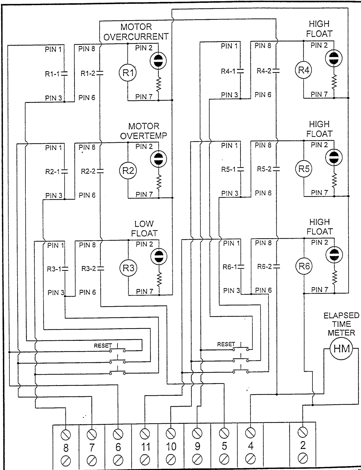
Figure 4-9. Electrical Configuration of an Example Annunciator Panel
