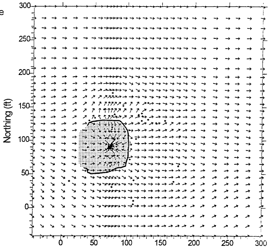
Figure 3-12A. Simulated Flow Vectors for the Oil Phase
