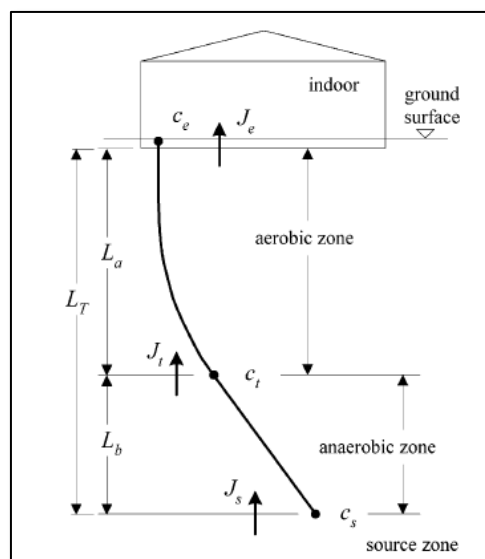
Conceptual Model for Vadose Zone Oxygen-Limited Biodegradation 161
