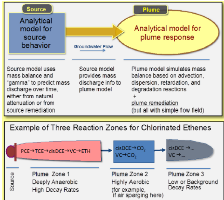
Overview of REMChlor Model
