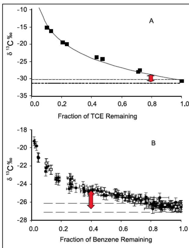
Degradation of (A) TCE and (B) benzene by enrichment cultures. The stable carbon isotope ratios in the substrate that remains after biodegradation are plotted against the fraction of the original concentration remaining. Data for TCE degradation are after Sherwood Lollar et al. 72 and for benzene after Mancini et al. 81 . Dotted lines represent \pm 0.5 ‰ around the \delta^{13}\text{C} value of TCE and of benzene, respectively. The vertical solid red arrow represents the extent of fractionation necessary to recognize biodegradation in field data (2‰) 5 .
