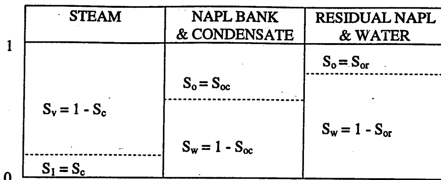
Figure I-2. Saturation Distributions
