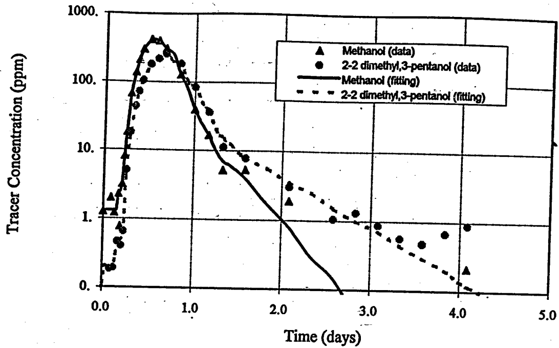
Figure 55a MLS24_YELLOW tracer response data and the corresponding fitting curves
