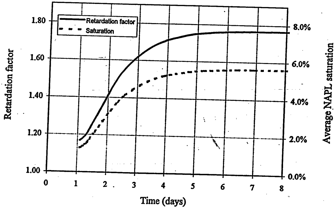
Figure 10b Estimated retardation factor and residual NAPL saturation based on tracer data at MLS21_BLUE
