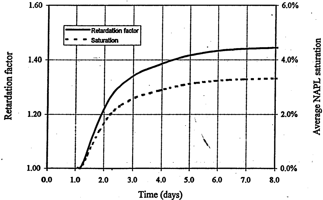
Figure 25b Estimated retardation factor and residual NAPL saturation based on tracer data at MLS22_BLUE
