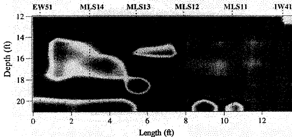
b) A cross-sectional view along the extraction well EW51.
