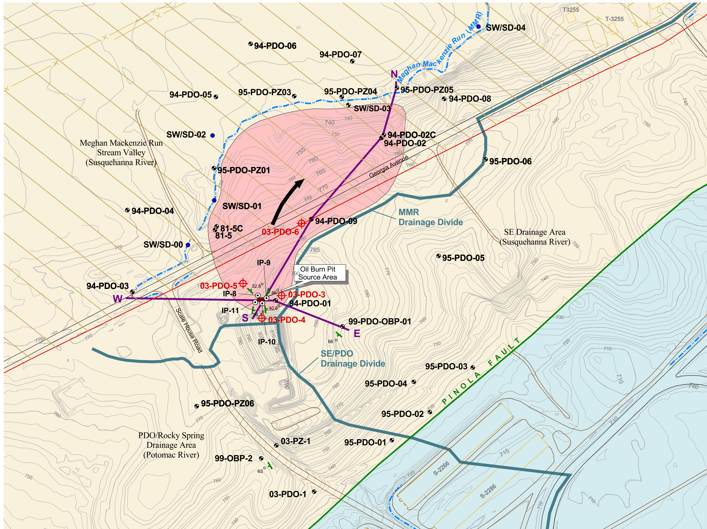
Figure 1 Location Map of Geologic Cross Sections and Newly Proposed Well Locations Letterkenny Army Depot
