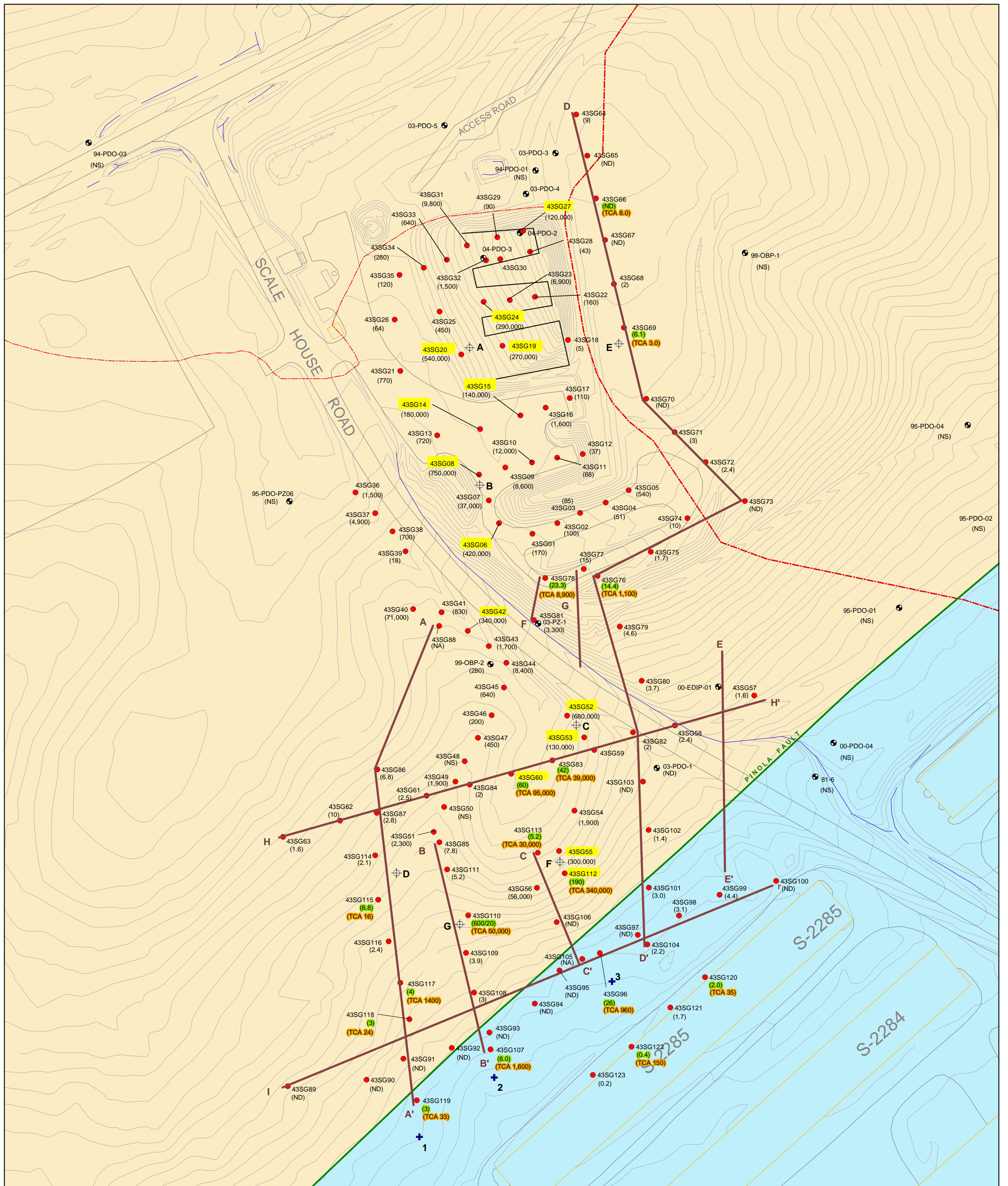
Figure 3 Soil Gas Results and Proposed Monitor Well Locations for Further Delineating the Extent of the OTL/TBR Area Groundwater Plume
