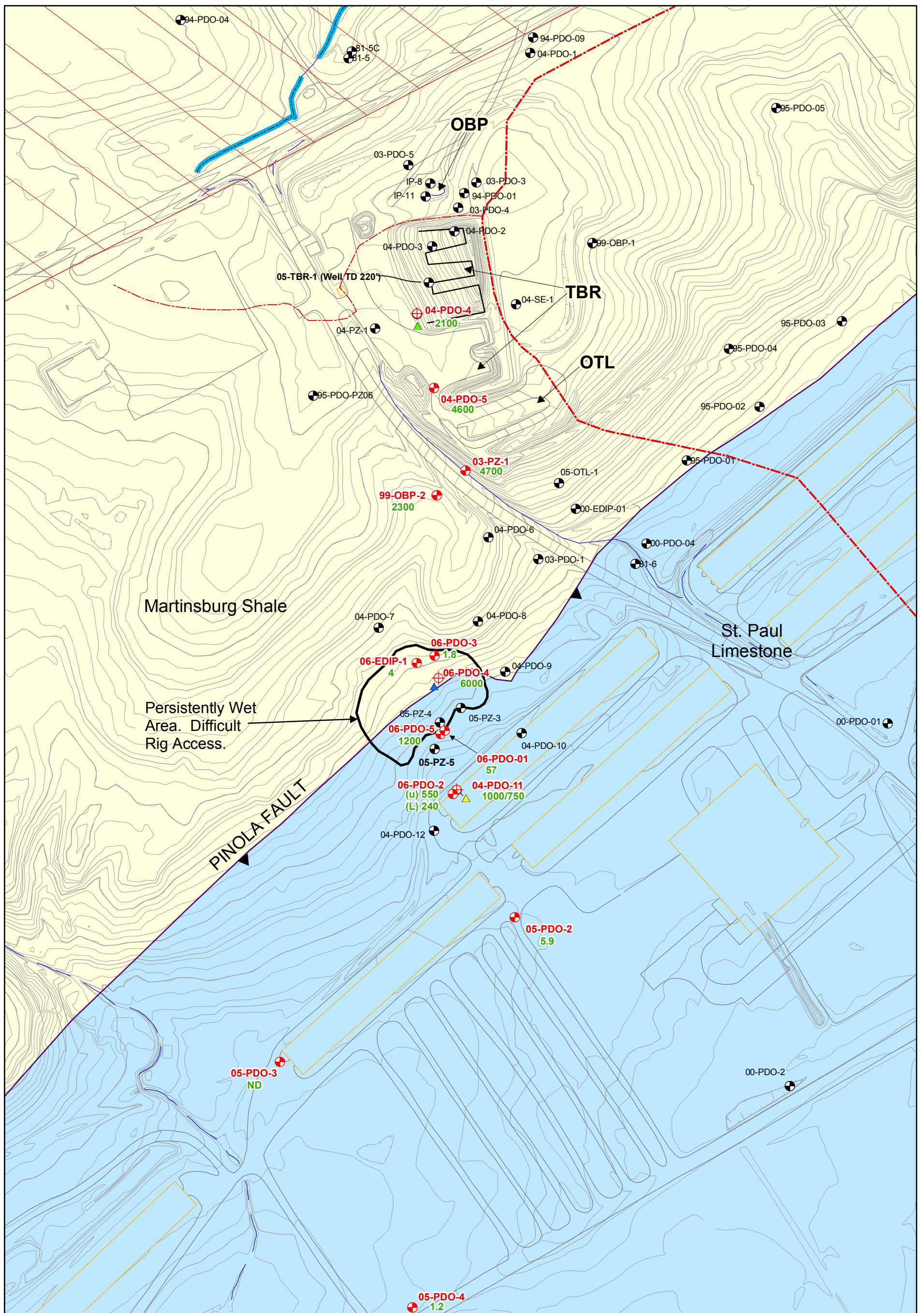
Figure 4 Dye Injection and Sampling Locations in the Upper PDO/Pinola Fault Area Showing Recent 1,1,1-TCA Concentrations
