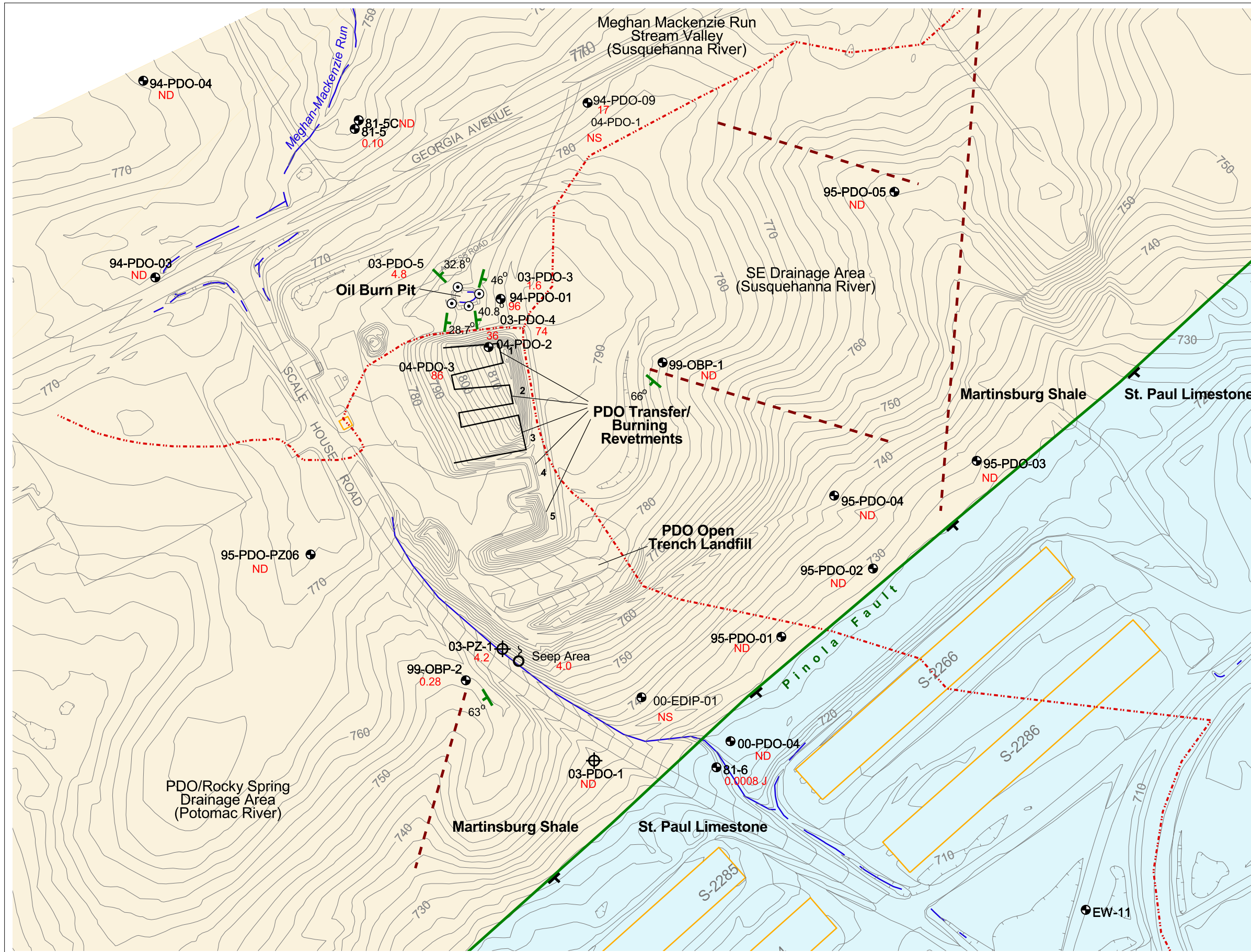
Figure 2 Recent/Historical 1,1,1-TCA Groundwater Concentrations at the Oil Burn Pit, Transfer Burning Revetments and Open Trench Landfill Area
