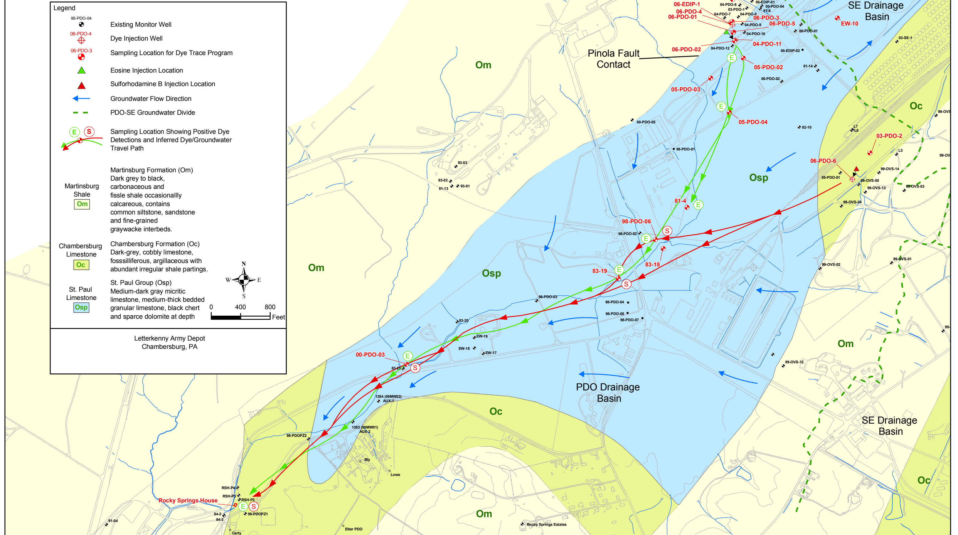
Figure 6 Upper PDO Dye Tracing Program Phase I Results 5 Dec 2006 - 22 Jan 2007
