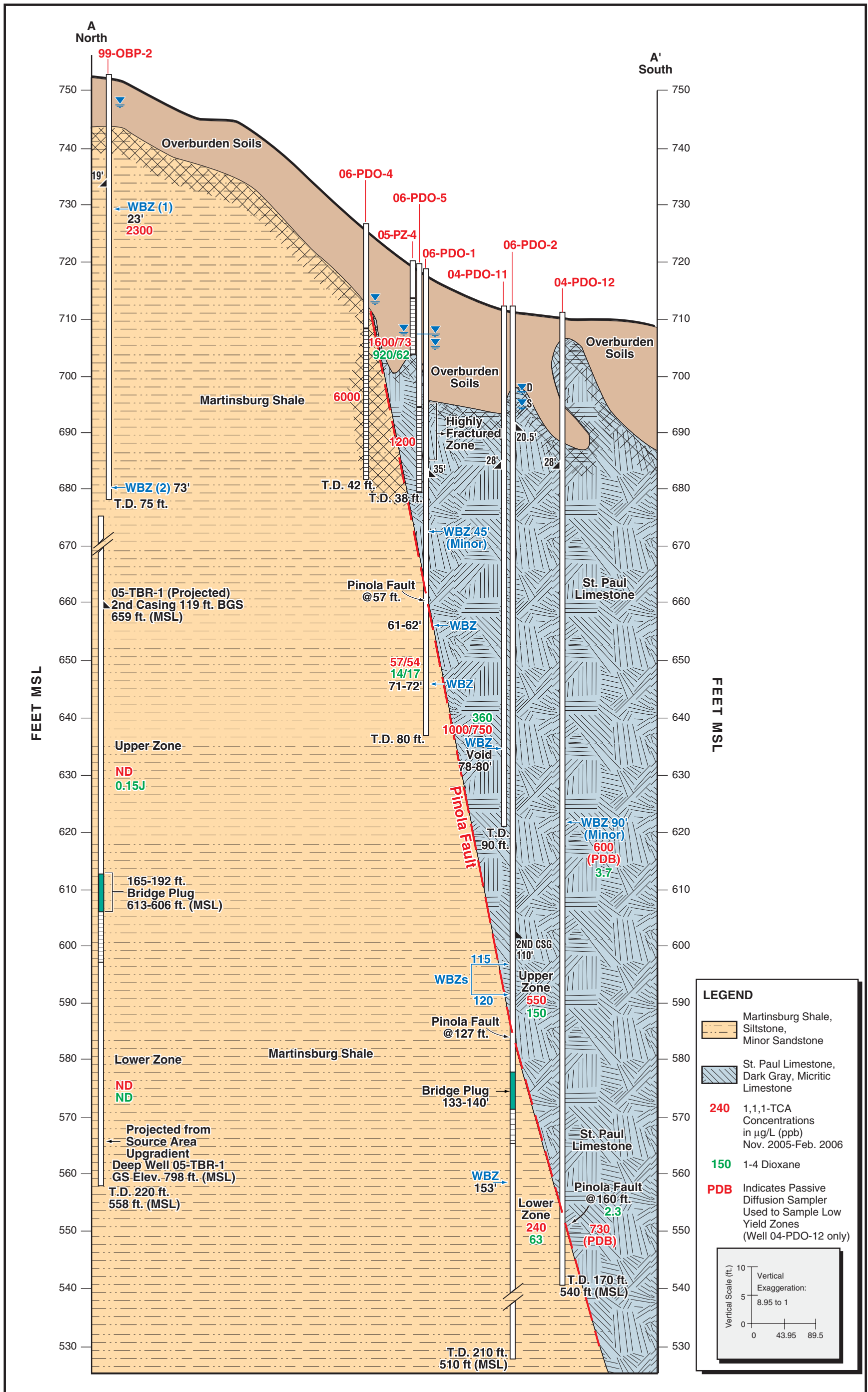
FIGURE 5 NORTH SOUTH HYDROGEOLOGIC CROSS-SECTION OF THE PINOLA FAULT AREA IN THE UPPER PDO - LETTERKENNY ARMY DEPOT, CHAMBERSBURG, PA
